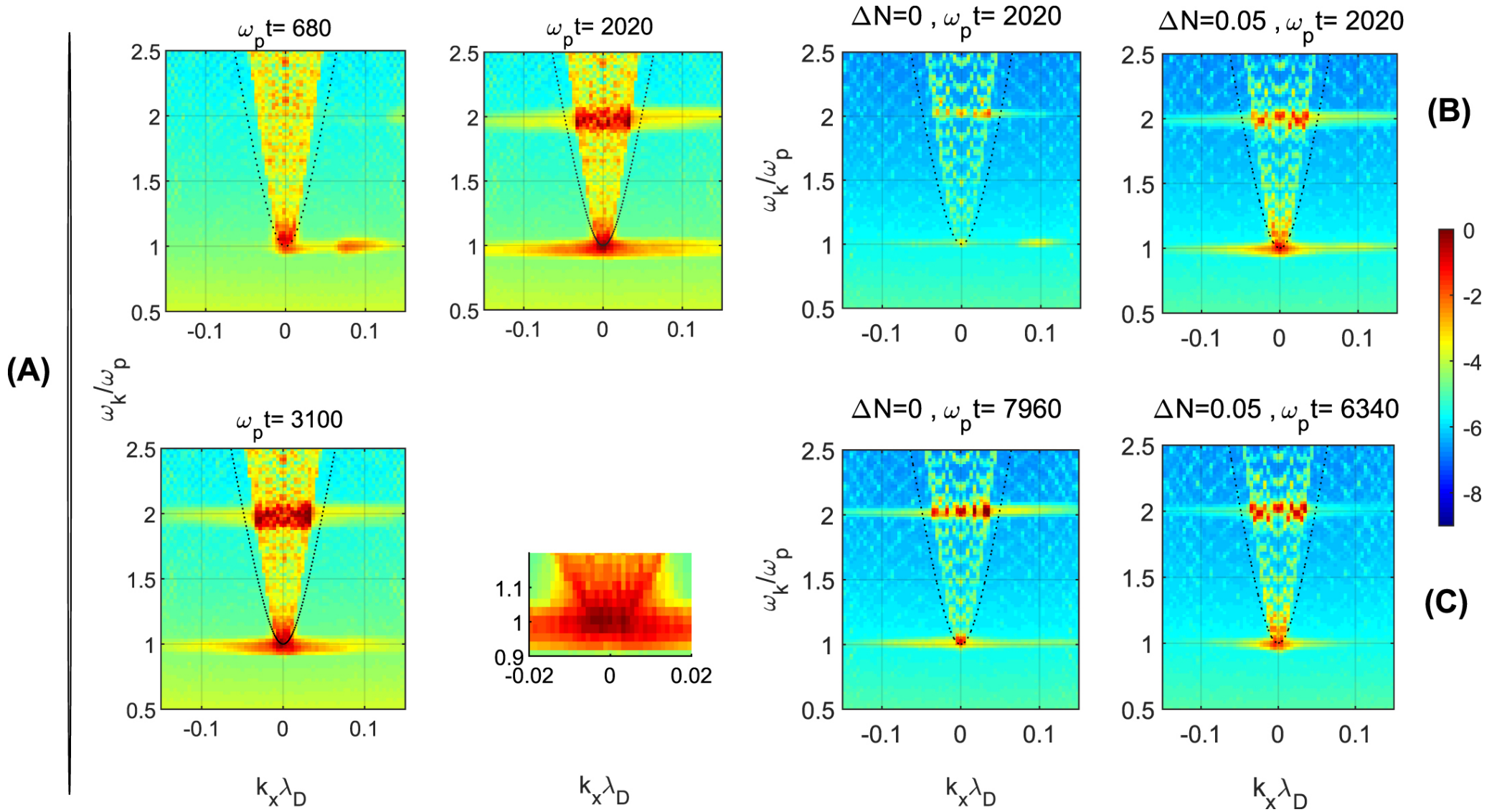
Figure 4. from Fundamental Electromagnetic Emissions by a Weak Electron Beam in Solar Wind Plasmas with Density Fluctuations null 2022 APJL 924 L24 doi:10.3847/2041-8213/ac46a7 https://dx.doi.org/10.3847/2041-8213/ac46a7 © 2022. The Author(s). Published by the American Astronomical Society.
