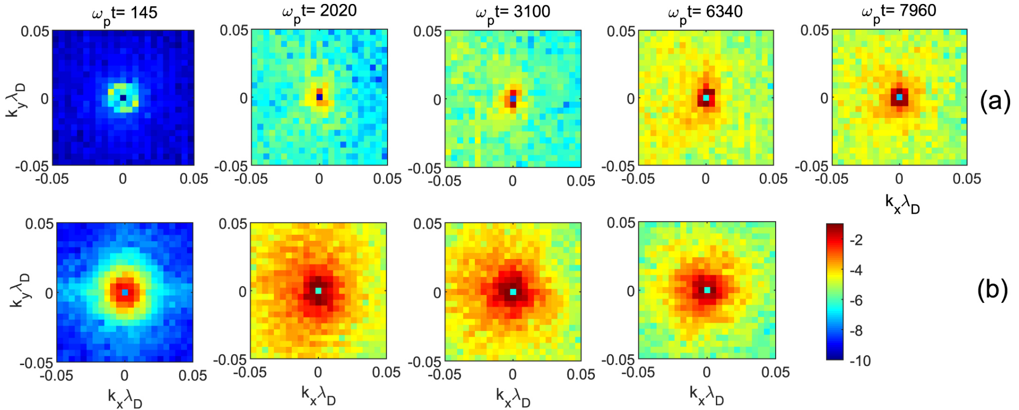
Figure 3. from Fundamental Electromagnetic Emissions by a Weak Electron Beam in Solar Wind Plasmas with Density Fluctuations null 2022 APJL 924 L24 doi:10.3847/2041-8213/ac46a7 http://dx.doi.org/10.3847/2041-8213/ac46a7
