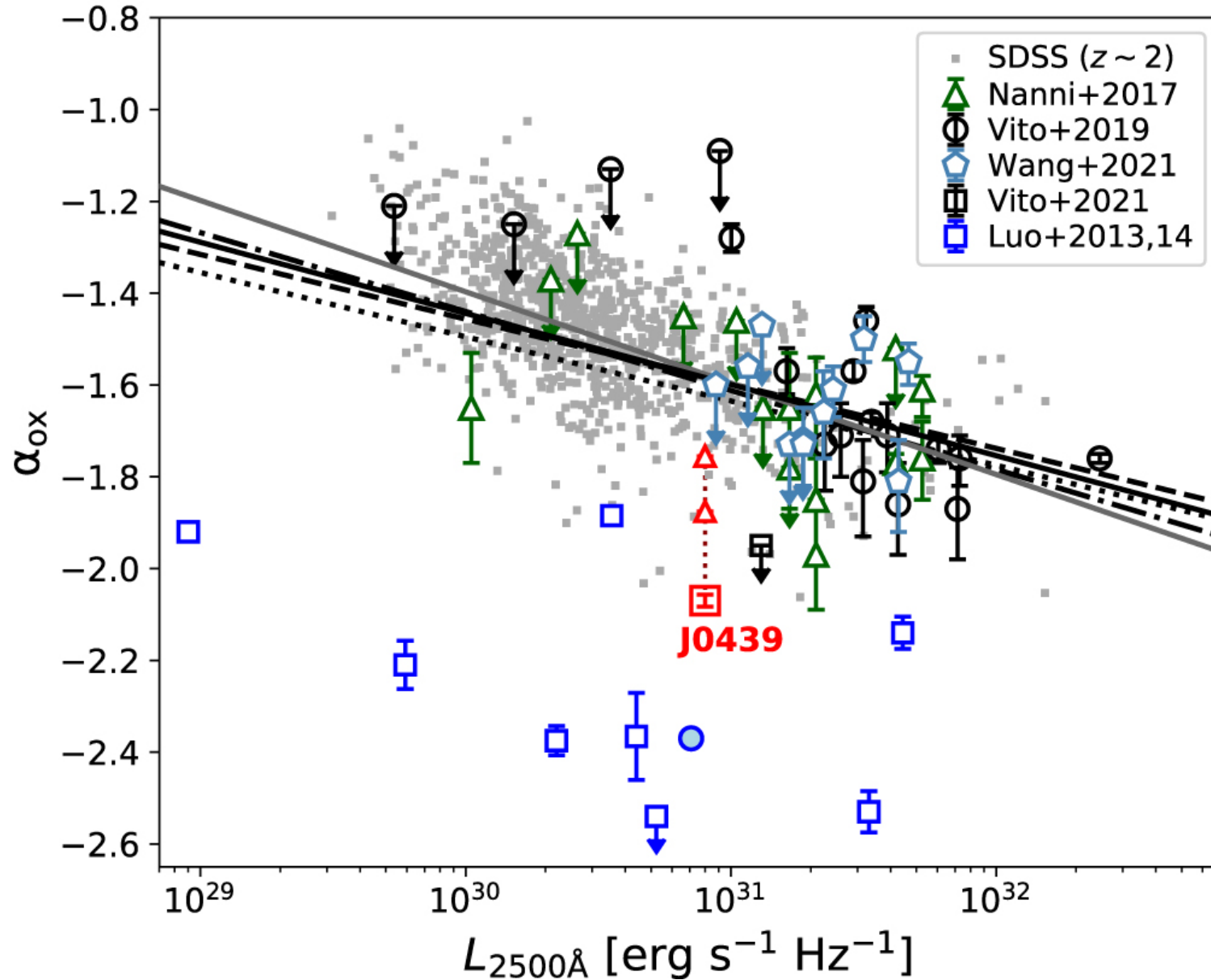
Figure 3. from Deep XMM-Newton Observations of an X-ray Weak Broad Absorption Line Quasar at z = 6.5 null 2022 APJL 924 L25 doi:10.3847/2041-8213/ac45f2 http://dx.doi.org/10.3847/2041-8213/ac45f2 © 2022. The Author(s). Published by the American Astronomical Society.
