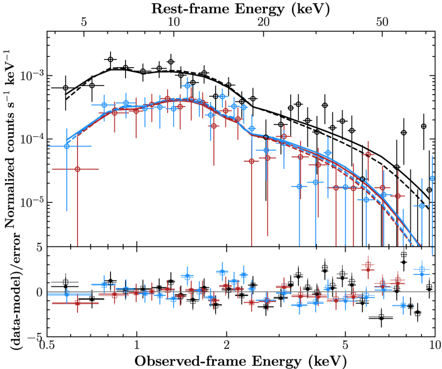
Figure 2. from Deep XMM-Newton Observations of an X-ray Weak Broad Absorption Line Quasar at z = 6.5 null 2022 APJL 924 L25 doi:10.3847/2041-8213/ac45f2 http://dx.doi.org/10.3847/2041-8213/ac45f2 © 2022. The Author(s). Published by the American Astronomical Society.
