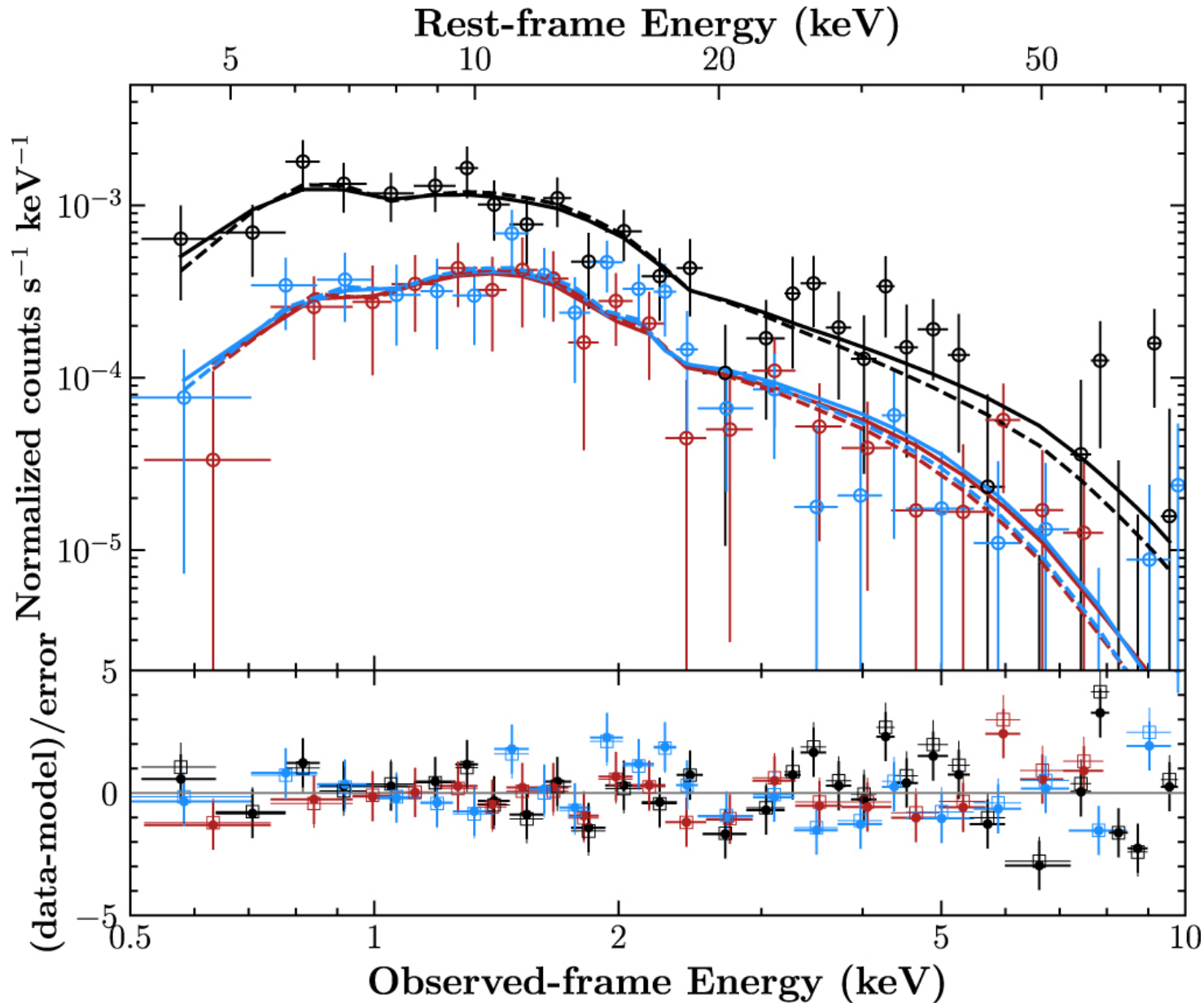
Figure 2. from Deep XMM-Newton Observations of an X-ray Weak Broad Absorption Line Quasar at z = 6.5 null 2022 APJL 924 L25 doi:10.3847/2041-8213/ac45f2 https://dx.doi.org/10.3847/2041-8213/ac45f2 © 2022. The Author(s). Published by the American Astronomical Society.
