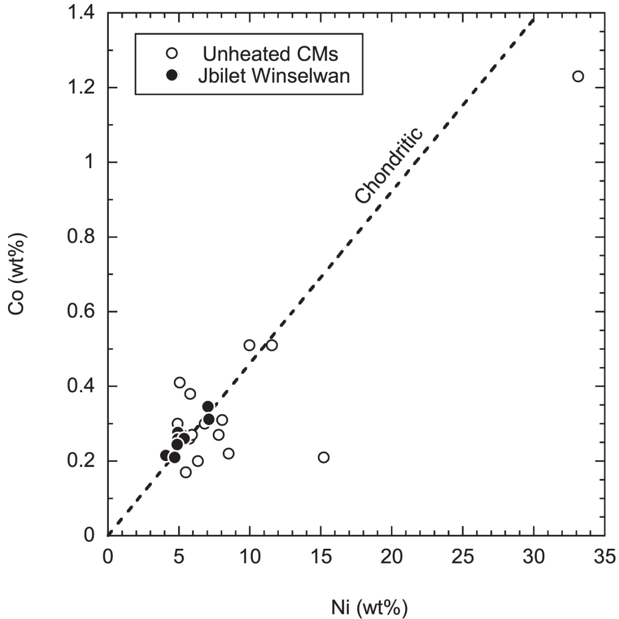
Figure A4. from Hydrothermal Activities on C-Complex Asteroids Induced by Radioactivity null 2022 APJL 924 L16 doi:10.3847/2041-8213/ac448f http://dx.doi.org/10.3847/2041-8213/ac448f © 2022. The Author(s). Published by the American Astronomical Society.
