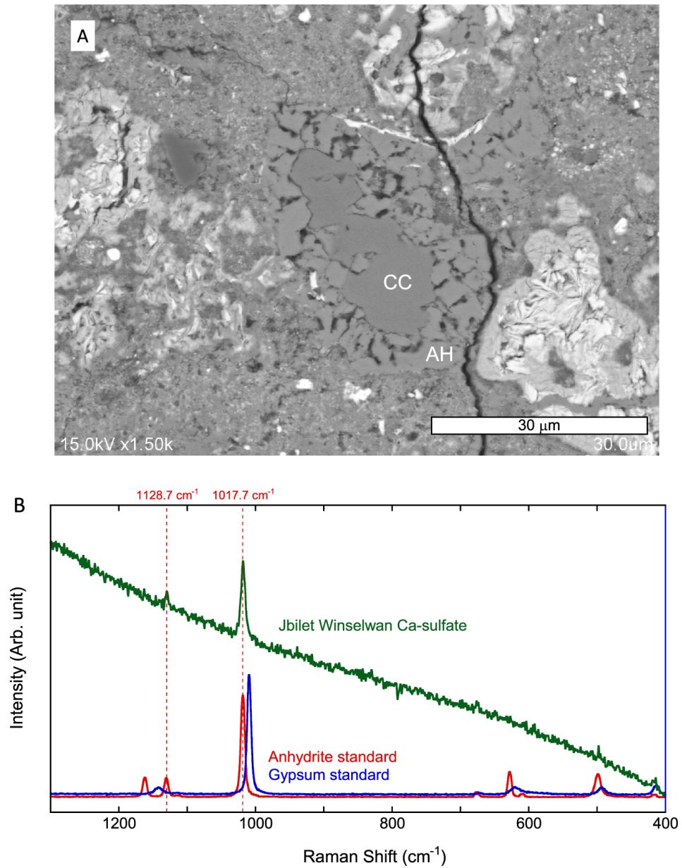
Figure 3. from Hydrothermal Activities on C-Complex Asteroids Induced by Radioactivity null 2022 APJL 924 L16 doi:10.3847/2041-8213/ac448f http://dx.doi.org/10.3847/2041-8213/ac448f © 2022. The Author(s). Published by the American Astronomical Society.
