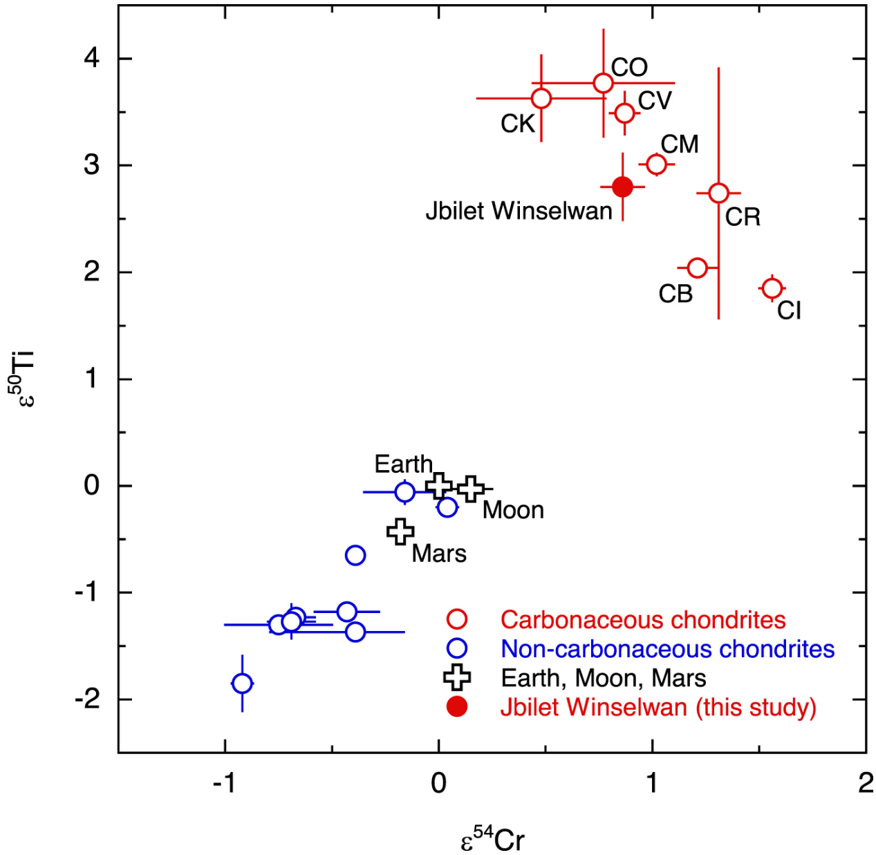
Figure 1. from Hydrothermal Activities on C-Complex Asteroids Induced by Radioactivity null 2022 APJL 924 L16 doi:10.3847/2041-8213/ac448f http://dx.doi.org/10.3847/2041-8213/ac448f © 2022. The Author(s). Published by the American Astronomical Society.
