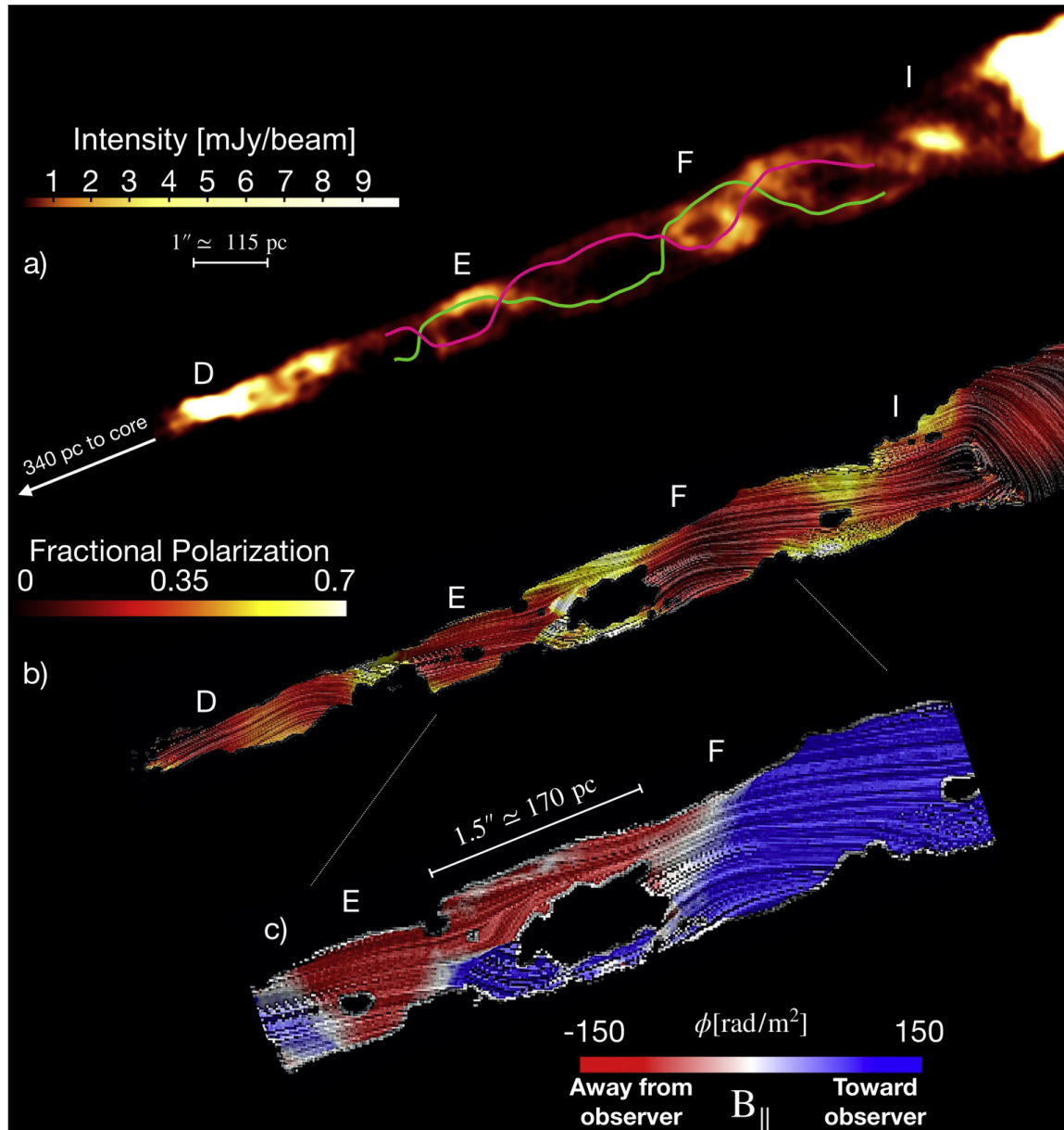
Figure 2. from Reading M87's DNA: A Double Helix Revealing a Large-scale Helical Magnetic Field null 2021 APJL 923 L5 doi:10.3847/2041-8213/ac3a88 https://dx.doi.org/10.3847/2041-8213/ac3a88 © 2021. The Author(s). Published by the American Astronomical Society.
