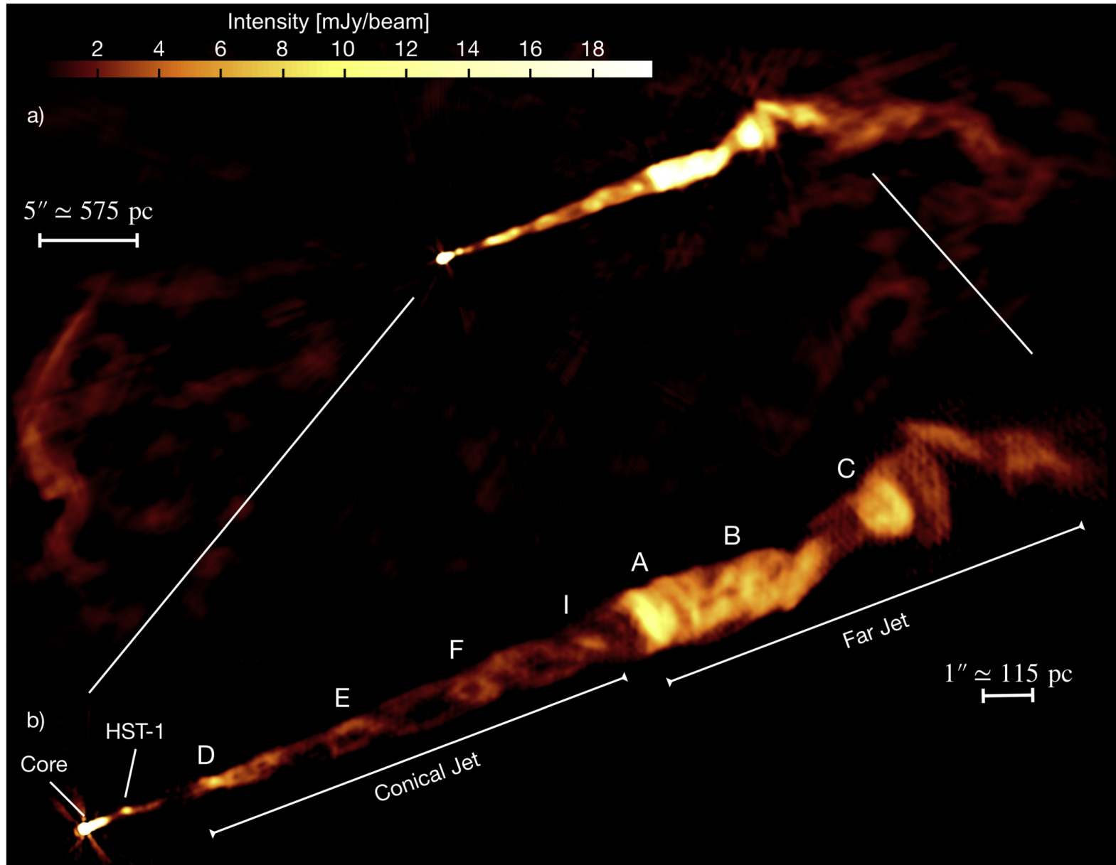
Figure 1. from Reading M87's DNA: A Double Helix Revealing a Large-scale Helical Magnetic Field null 2021 APJL 923 L5 doi:10.3847/2041-8213/ac3a88 https://dx.doi.org/10.3847/2041-8213/ac3a88 © 2021. The Author(s). Published by the American Astronomical Society.
