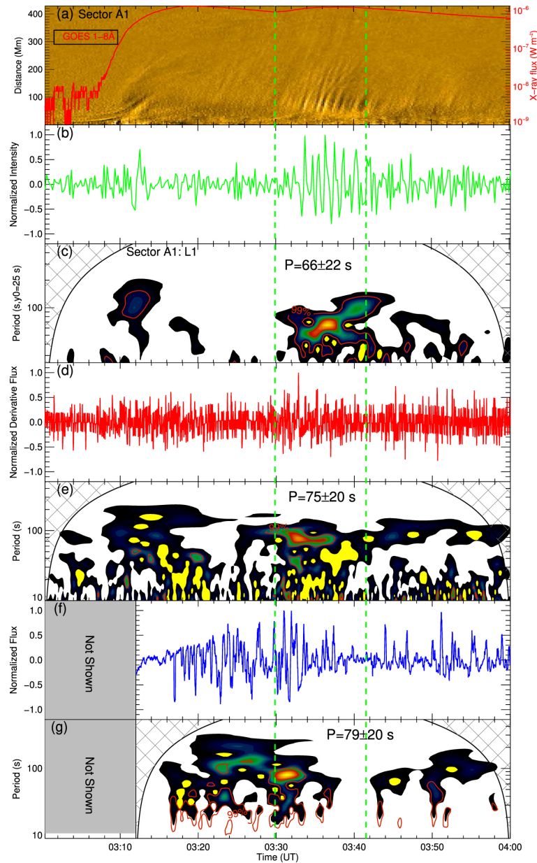
Figure 3. from Diagnosing a Solar Flaring Core with Bidirectional Quasi-periodic Fast Propagating Magnetoacoustic Waves null 2021 APJL 908 L37 doi:10.3847/2041-8213/abdfce https://dx.doi.org/10.3847/2041-8213/abdfce
