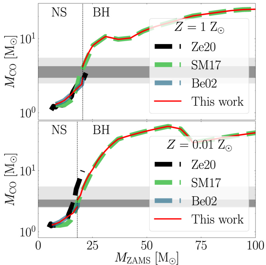
Figure 6. from Dynamical Formation of the GW190814 Merger null 2021 APJL 908 L38 doi:10.3847/2041-8213/abdfcd http://dx.doi.org/10.3847/2041-8213/abdfcd © 2021. The American Astronomical Society. All rights reserved.
