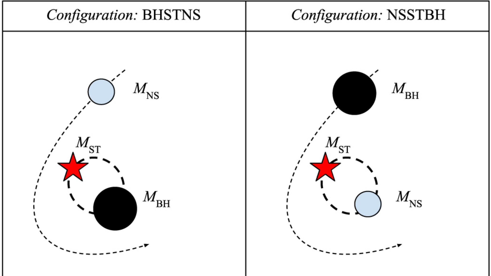
Figure 1. from Dynamical Formation of the GW190814 Merger null 2021 APJL 908 L38 doi:10.3847/2041-8213/abdfcd http://dx.doi.org/10.3847/2041-8213/abdfcd © 2021. The American Astronomical Society. All rights reserved.
