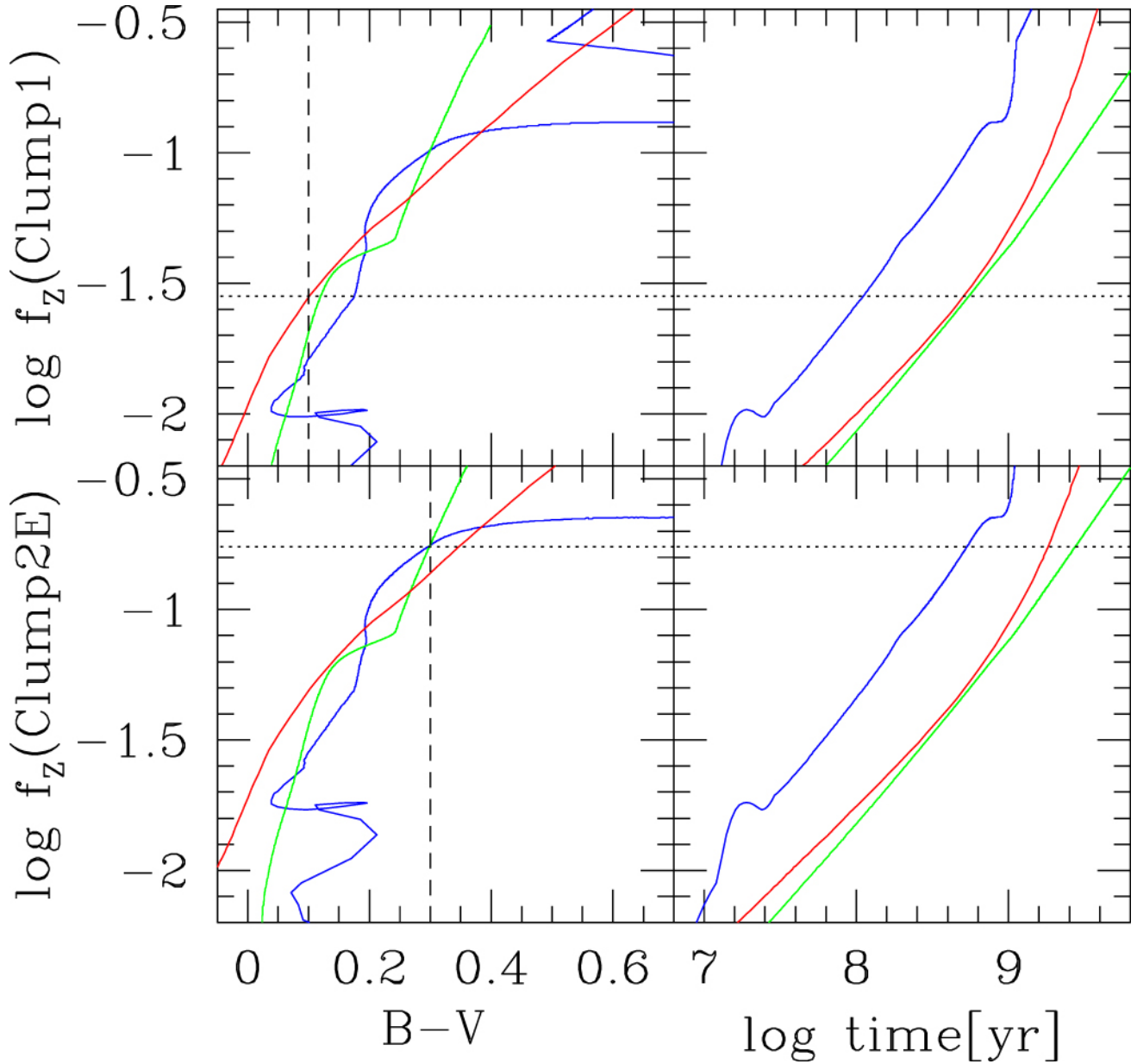
Figure 3. from Heavy Elements Unveil the Non-primordial Origin of the Giant H I Ring in Leo null 2021 APJL 908 L39 doi:10.3847/2041-8213/abdf64 http://dx.doi.org/10.3847/2041-8213/abdf64 © 2021. The American Astronomical Society. All rights reserved.
