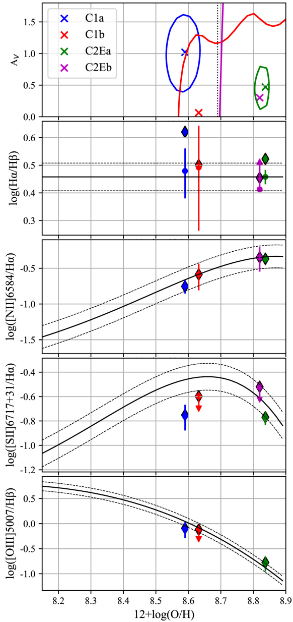
Figure 2. from Heavy Elements Unveil the Non-primordial Origin of the Giant H I Ring in Leo null 2021 APJL 908 L39 doi:10.3847/2041-8213/abdf64 http://dx.doi.org/10.3847/2041-8213/abdf64 © 2021. The American Astronomical Society. All rights reserved.
