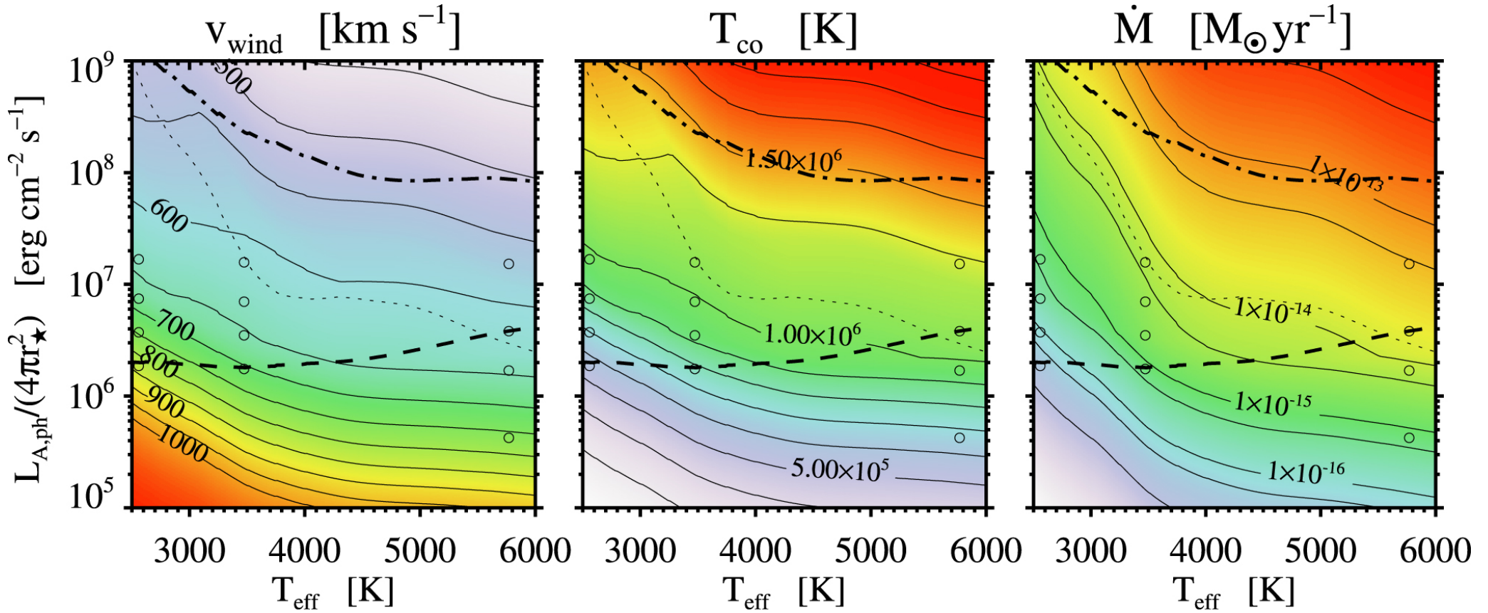
Figure 5. from Nonlinear Alfvén Wave Model of Stellar Coronae and Winds from the Sun to M Dwarfs null 2021 APJL 906 L13 doi:10.3847/2041-8213/abd3a9 http://dx.doi.org/10.3847/2041-8213/abd3a9 © 2021. The American Astronomical Society. All rights reserved.
