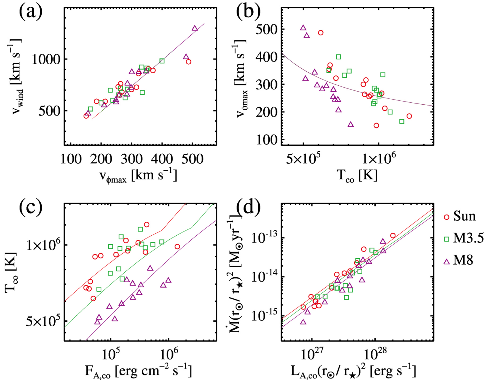
Figure 4. from Nonlinear Alfvén Wave Model of Stellar Coronae and Winds from the Sun to M Dwarfs null 2021 APJL 906 L13 doi:10.3847/2041-8213/abd3a9 http://dx.doi.org/10.3847/2041-8213/abd3a9 © 2021. The American Astronomical Society. All rights reserved.
