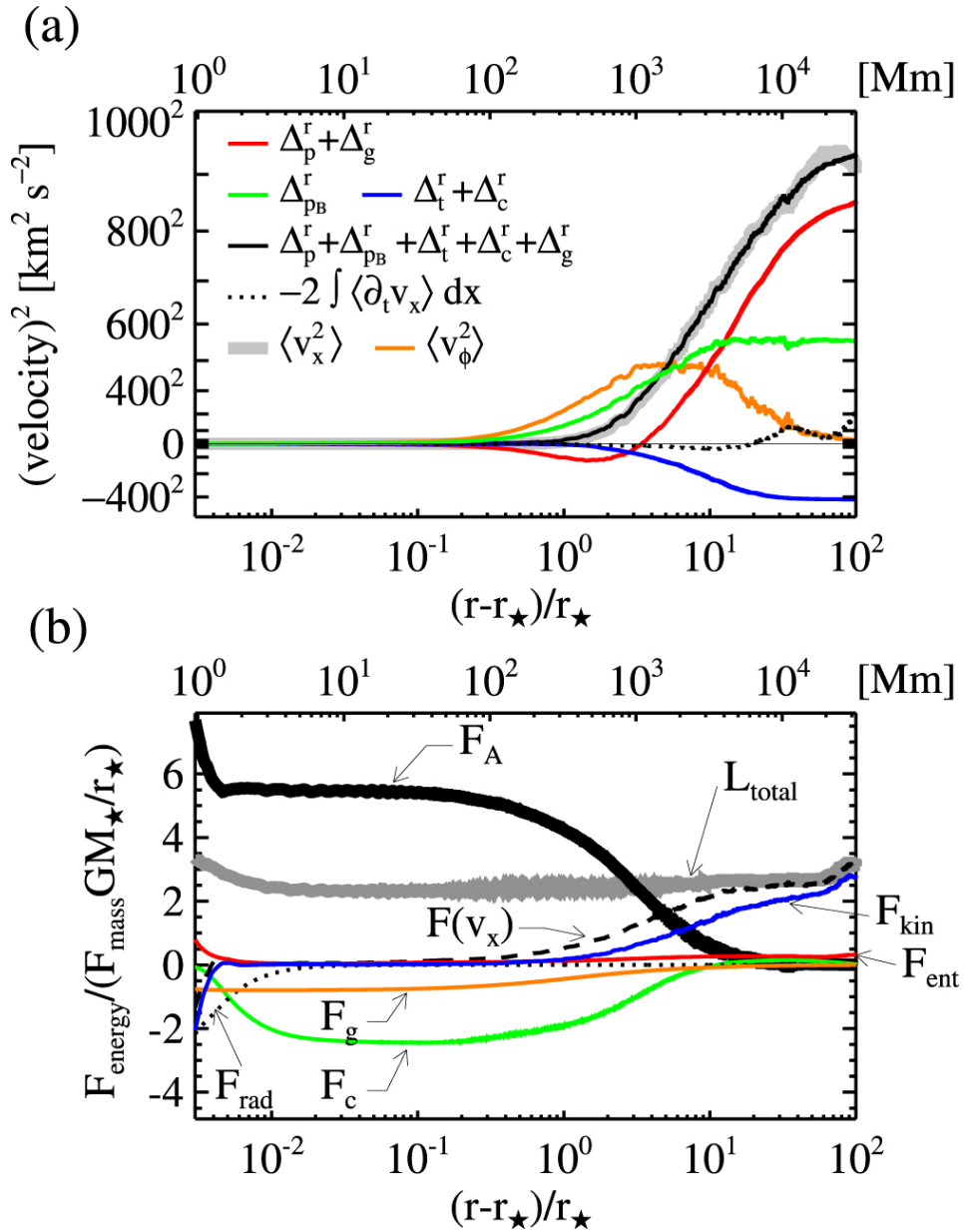
Figure 3. from Nonlinear Alfvén Wave Model of Stellar Coronae and Winds from the Sun to M Dwarfs null 2021 APJL 906 L13 doi:10.3847/2041-8213/abd3a9 http://dx.doi.org/10.3847/2041-8213/abd3a9 © 2021. The American Astronomical Society. All rights reserved.
