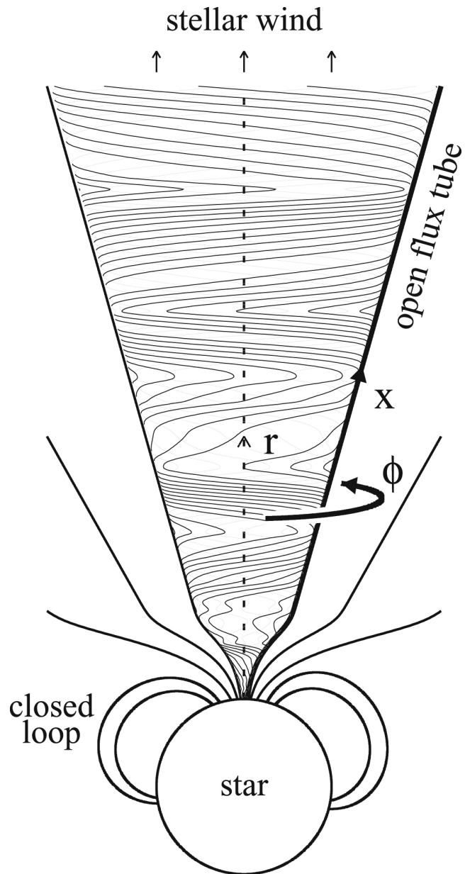
Figure 1. from Nonlinear Alfvén Wave Model of Stellar Coronae and Winds from the Sun to M Dwarfs null 2021 APJL 906 L13 doi:10.3847/2041-8213/abd3a9 http://dx.doi.org/10.3847/2041-8213/abd3a9 © 2021. The American Astronomical Society. All rights reserved.
