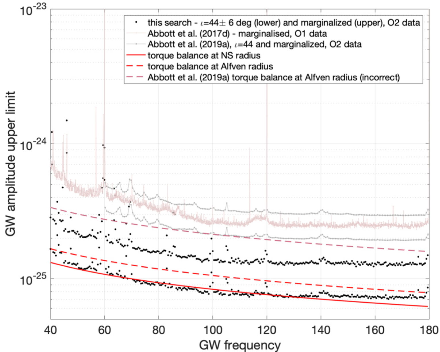
Figure 1. from Search for Continuous Gravitational Waves from Scorpius X-1 in LIGO O2 Data null 2021 APJL 906 L14 doi:10.3847/2041-8213/abd256 https://dx.doi.org/10.3847/2041-8213/abd256 © 2021. The Author(s). Published by the American Astronomical Society.
