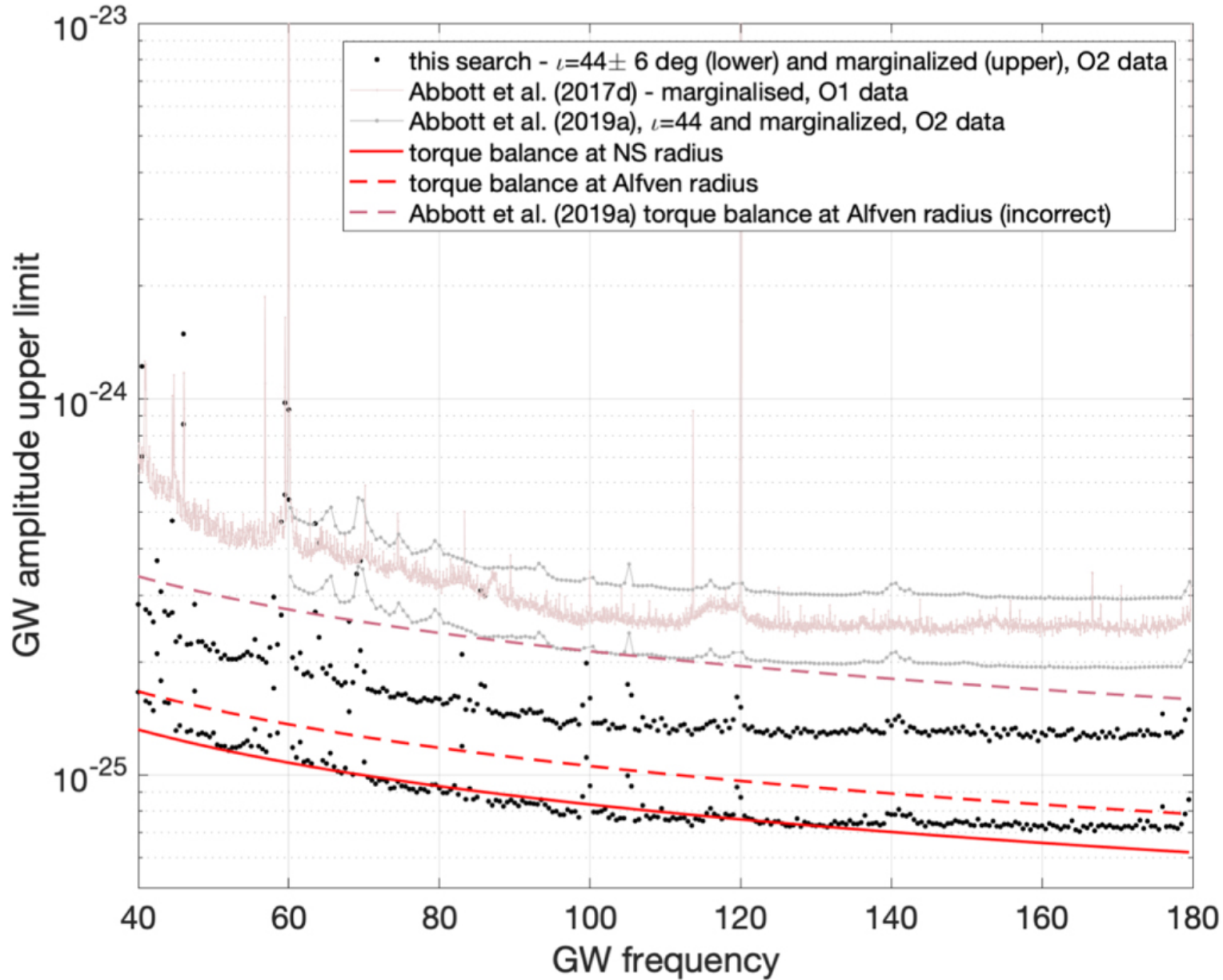
Figure 1. from Search for Continuous Gravitational Waves from Scorpius X-1 in LIGO O2 Data null 2021 APJL 906 L14 doi:10.3847/2041-8213/abd256 http://dx.doi.org/10.3847/2041-8213/abd256 © 2021. The Author(s). Published by the American Astronomical Society.
