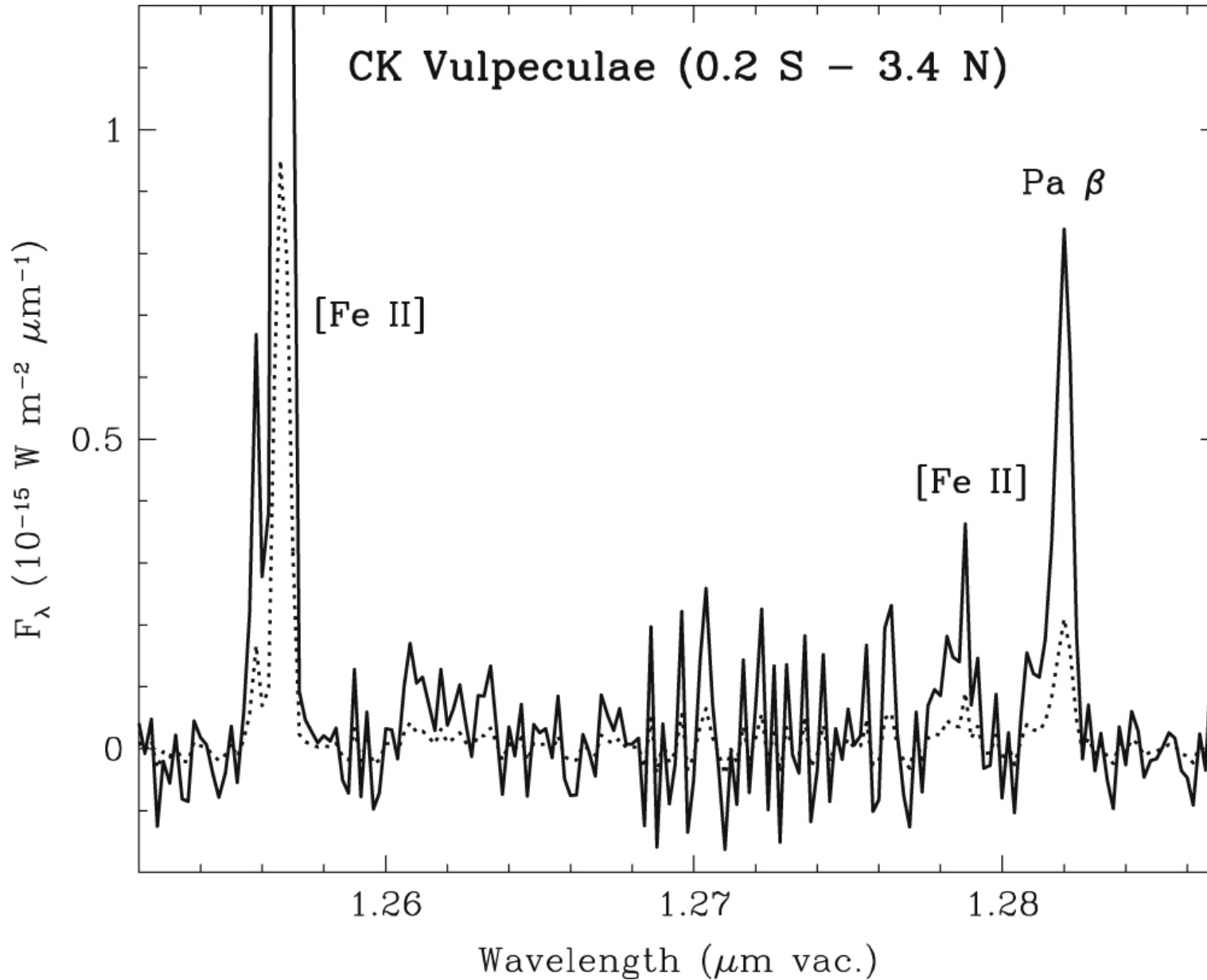
Figure 3. from Near-infrared Spectroscopy of CK Vulpeculae: Revealing a Remarkably Powerful Blast from the Past null 2020 APJL 904 L23 doi:10.3847/2041-8213/abc885 https://dx.doi.org/10.3847/2041-8213/abc885 © 2020. The American Astronomical Society. All rights reserved.
