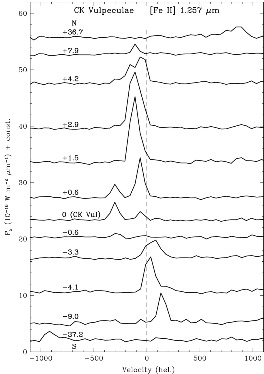
Figure 2. from Near-infrared Spectroscopy of CK Vulpeculae: Revealing a Remarkably Powerful Blast from the Past null 2020 APJL 904 L23 doi:10.3847/2041-8213/abc885 https://dx.doi.org/10.3847/2041-8213/abc885 © 2020. The American Astronomical Society. All rights reserved.
