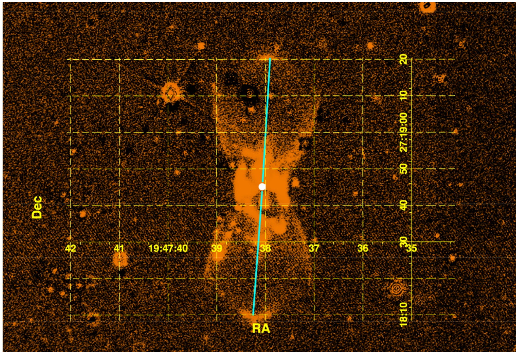
Figure 1. from Near-infrared Spectroscopy of CK Vulpeculae: Revealing a Remarkably Powerful Blast from the Past null 2020 APJL 904 L23 doi:10.3847/2041-8213/abc885 https://dx.doi.org/10.3847/2041-8213/abc885 © 2020. The American Astronomical Society. All rights reserved.
