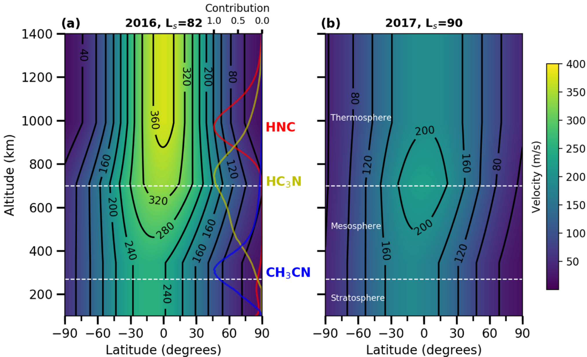
Figure 4. from Detection of Dynamical Instability in Titan's Thermospheric Jet null 2020 APJL 904 L12 doi:10.3847/2041-8213/abc688 http://dx.doi.org/10.3847/2041-8213/abc688 © 2020. The American Astronomical Society. All rights reserved.
