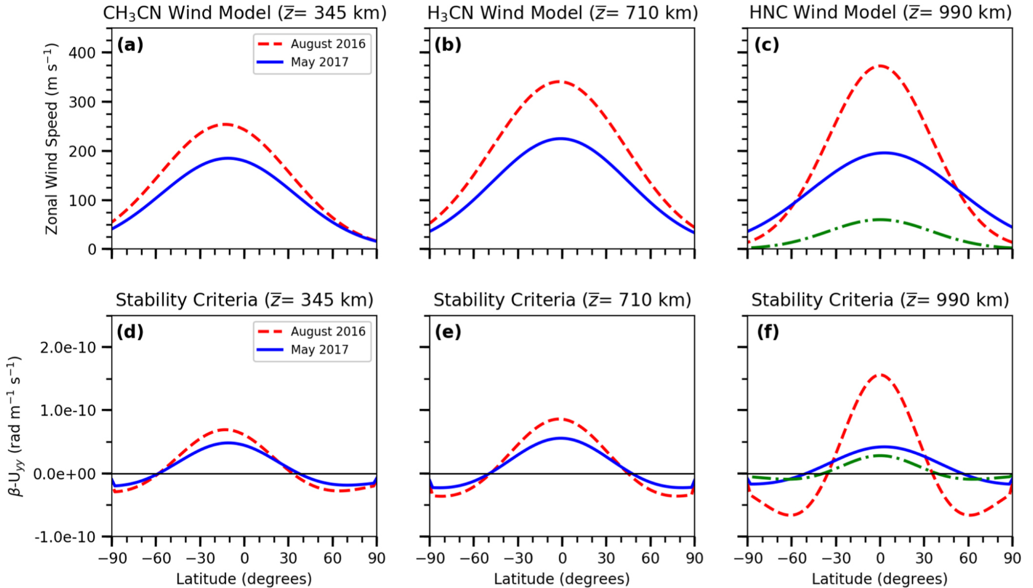
Figure 3. from Detection of Dynamical Instability in Titan's Thermospheric Jet null 2020 APJL 904 L12 doi:10.3847/2041-8213/abc688 http://dx.doi.org/10.3847/2041-8213/abc688 © 2020. The American Astronomical Society. All rights reserved.
