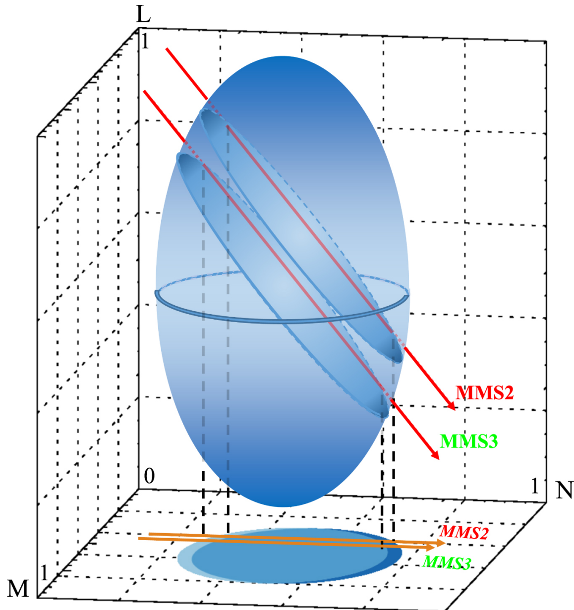
Figure 5. from Three-dimensional Geometry of the Electron-scale Magnetic Hole in the Solar Wind null 2020 APJL 904 L11 doi:10.3847/2041-8213/abc553 http://dx.doi.org/10.3847/2041-8213/abc553 © 2020. The American Astronomical Society. All rights reserved.
