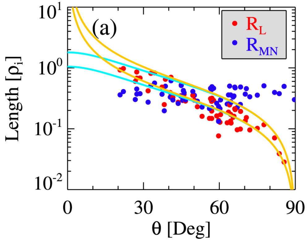
Figure 4. from Three-dimensional Geometry of the Electron-scale Magnetic Hole in the Solar Wind null 2020 APJL 904 L11 doi:10.3847/2041-8213/abc553 http://dx.doi.org/10.3847/2041-8213/abc553 © 2020. The American Astronomical Society. All rights reserved.
