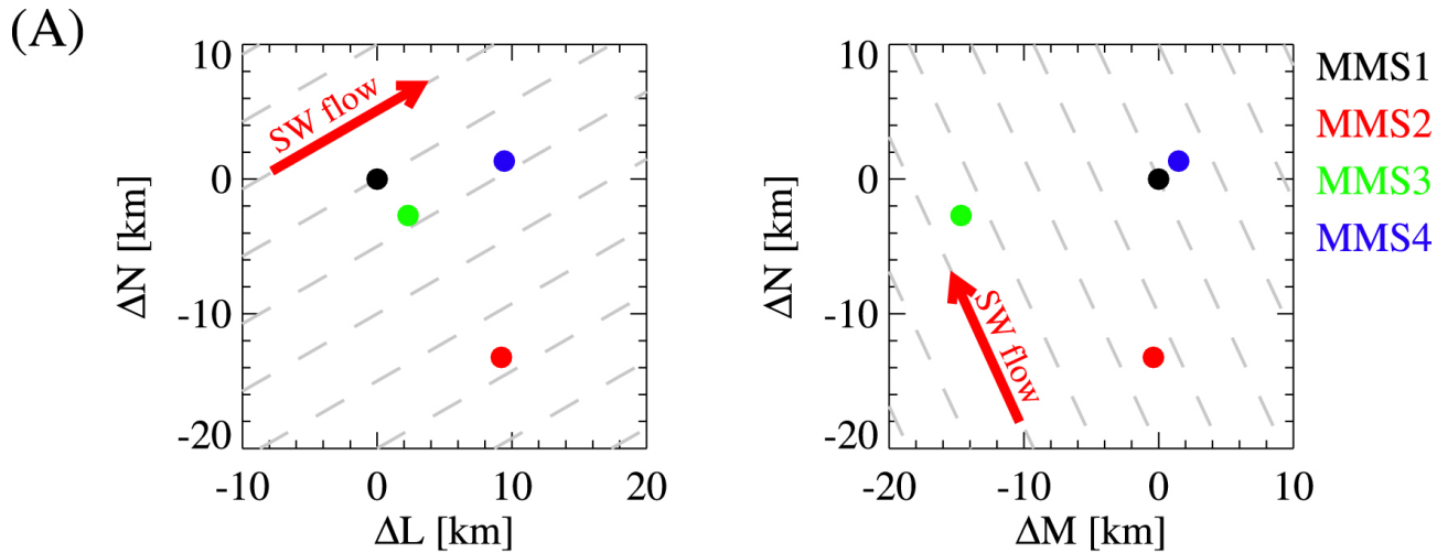
Figure 3. from Three-dimensional Geometry of the Electron-scale Magnetic Hole in the Solar Wind null 2020 APJL 904 L11 doi:10.3847/2041-8213/abc553 http://dx.doi.org/10.3847/2041-8213/abc553 © 2020. The American Astronomical Society. All rights reserved.
