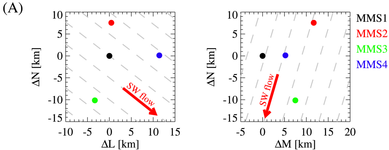
Figure 2. from Three-dimensional Geometry of the Electron-scale Magnetic Hole in the Solar Wind null 2020 APJL 904 L11 doi:10.3847/2041-8213/abc553 http://dx.doi.org/10.3847/2041-8213/abc553 © 2020. The American Astronomical Society. All rights reserved.
