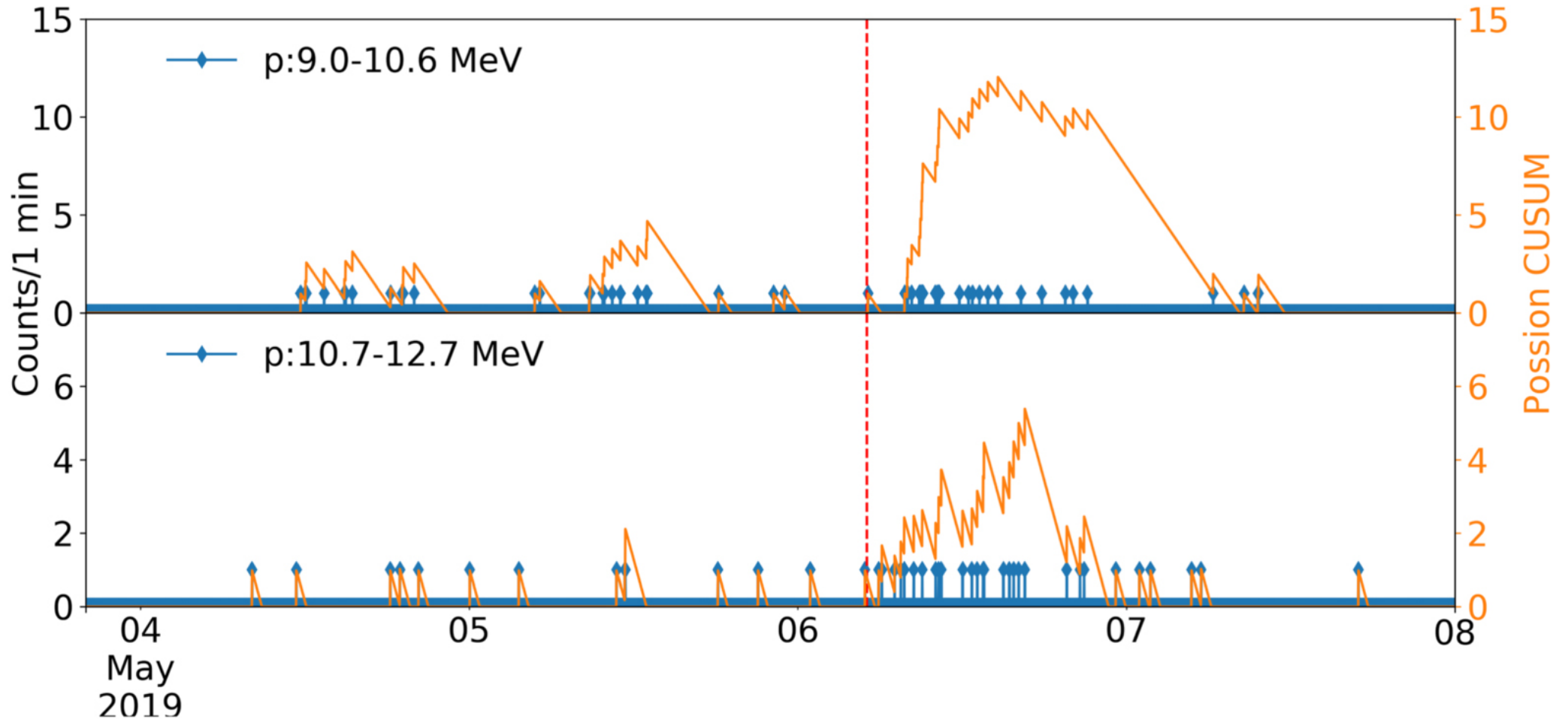
Figure 5. from First Solar Energetic Particles Measured on the Lunar Far-side null 2020 APJL 902 L30 doi:10.3847/2041-8213/abbccc http://dx.doi.org/10.3847/2041-8213/abbccc © 2020. The American Astronomical Society. All rights reserved.
