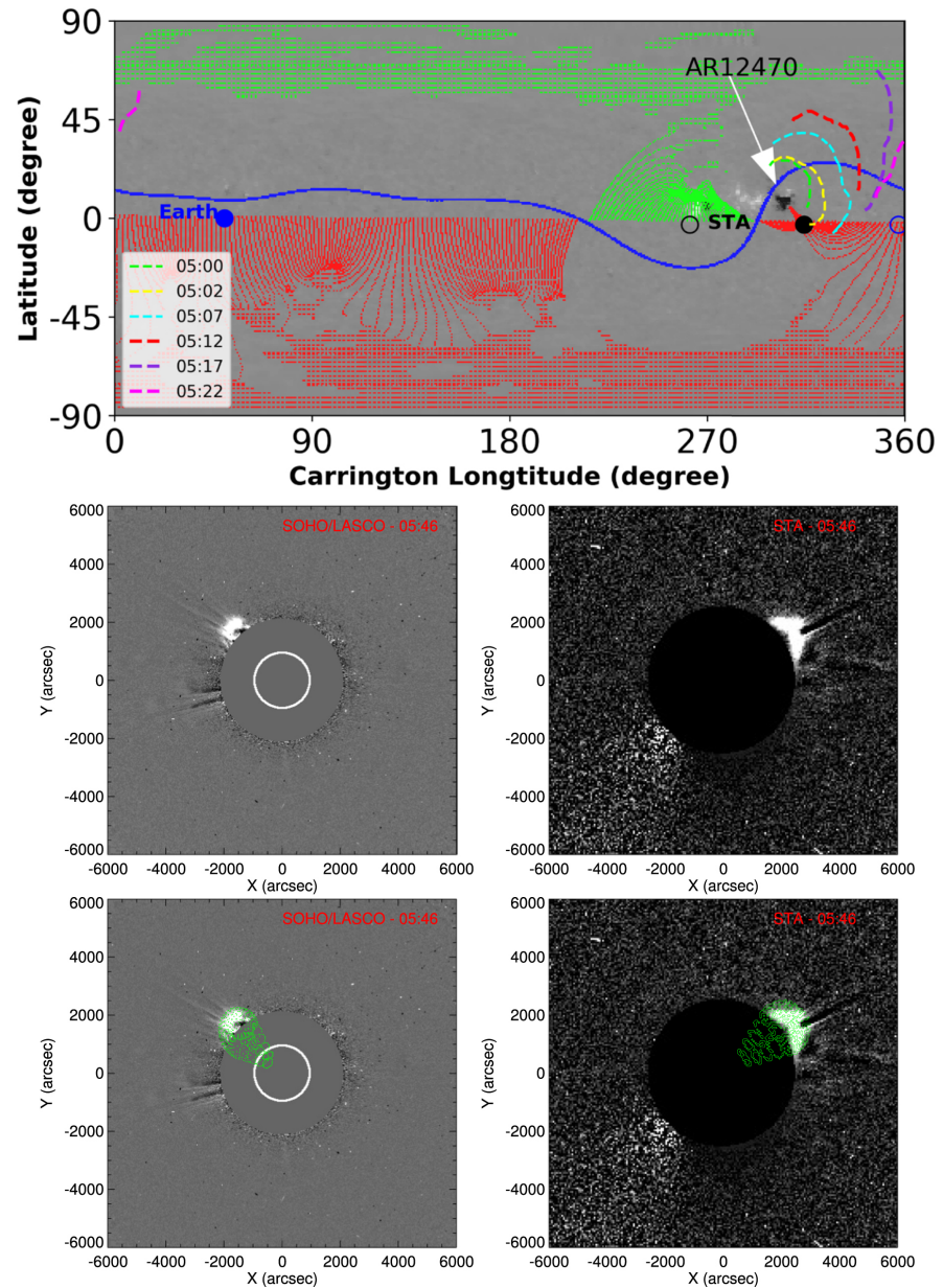
Figure 4. from First Solar Energetic Particles Measured on the Lunar Far-side null 2020 APJL 902 L30 doi:10.3847/2041-8213/abbccc https://dx.doi.org/10.3847/2041-8213/abbccc © 2020. The American Astronomical Society.
