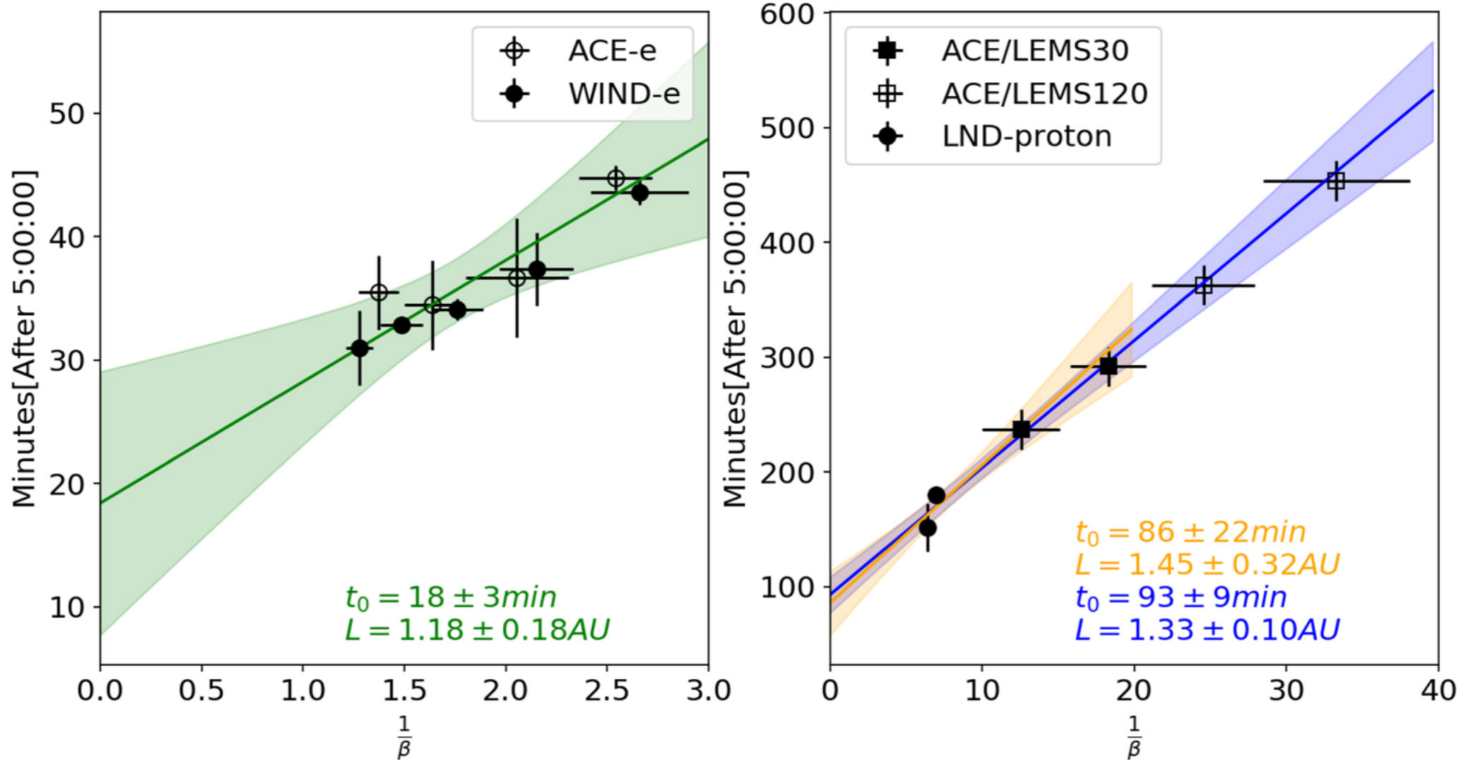
Figure 2. from First Solar Energetic Particles Measured on the Lunar Far-side null 2020 APJL 902 L30 doi:10.3847/2041-8213/abbccc http://dx.doi.org/10.3847/2041-8213/abbccc © 2020. The American Astronomical Society. All rights reserved.
