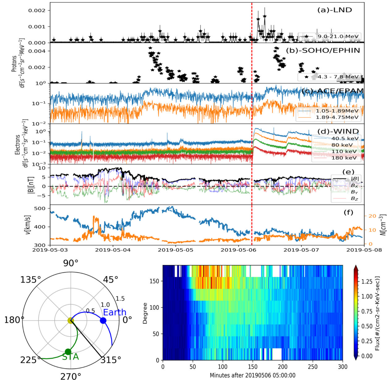
Figure 1. from First Solar Energetic Particles Measured on the Lunar Far-side null 2020 APJL 902 L30 doi:10.3847/2041-8213/abbccc https://dx.doi.org/10.3847/2041-8213/abbccc © 2020. The American Astronomical Society.
