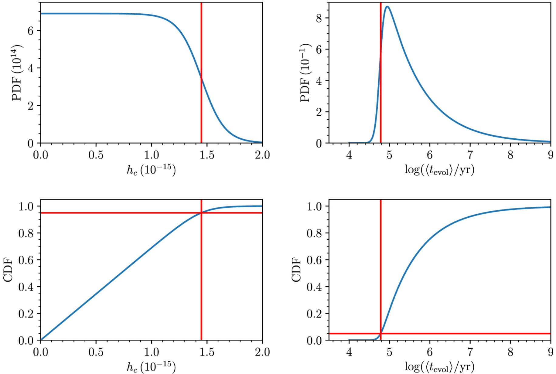
Figure 3. from Pulsar Timing Array Constraints on the Merger Timescale of Subparsec Supermassive Black Hole Binary Candidates null 2020 APJL 900 L42 doi:10.3847/2041-8213/abb2ab http://dx.doi.org/10.3847/2041-8213/abb2ab © 2020. The American Astronomical Society. All rights reserved.
