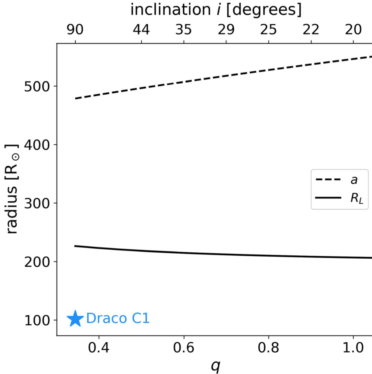
Figure 4. from Geometry of the Draco C1 Symbiotic Binary null 2020 APJL 900 L43 doi:10.3847/2041-8213/abb248 http://dx.doi.org/10.3847/2041-8213/abb248
