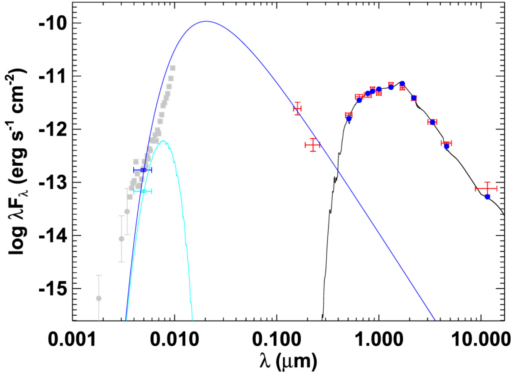
Figure 1. from Geometry of the Draco C1 Symbiotic Binary null 2020 APJL 900 L43 doi:10.3847/2041-8213/abb248 http://dx.doi.org/10.3847/2041-8213/abb248 © 2020. The American Astronomical Society. All rights reserved.
