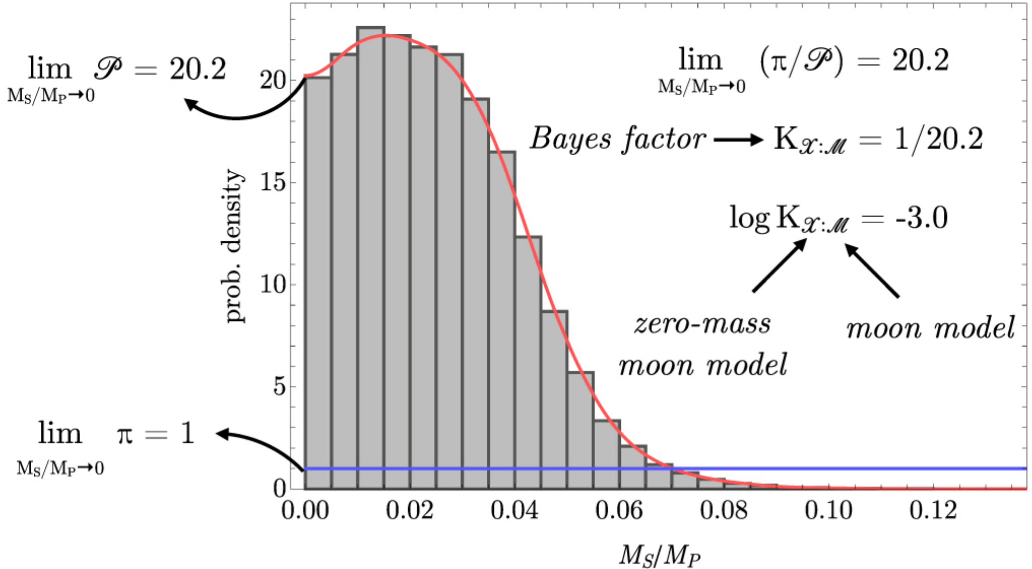
Figure 2. from An Independent Analysis of the Six Recently Claimed Exomoon Candidates null 2020 APJL 900 L44 doi:10.3847/2041-8213/abafa9 http://dx.doi.org/10.3847/2041-8213/abafa9 © 2020. The American Astronomical Society. All rights reserved.
