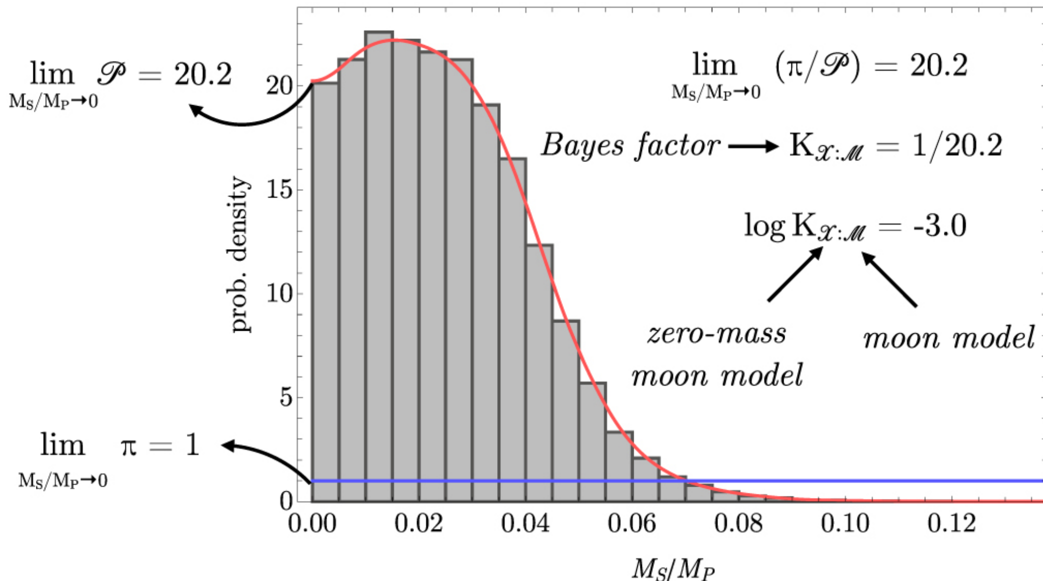
Figure 2. from An Independent Analysis of the Six Recently Claimed Exomoon Candidates null 2020 APJL 900 L44 doi:10.3847/2041-8213/abafa9 https://dx.doi.org/10.3847/2041-8213/abafa9 © 2020. The American Astronomical Society. All rights reserved.
