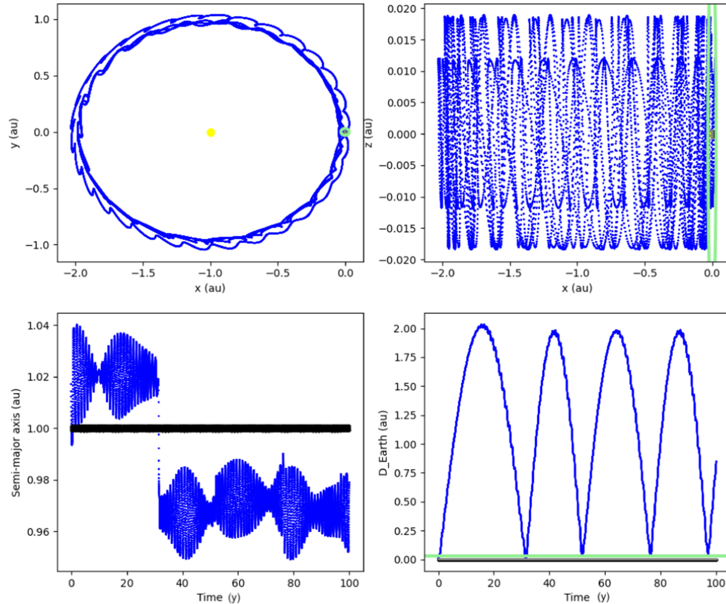
Figure 8. from Characterization of Temporarily Captured Minimoon 2020 CD3 by Keck Time-resolved Spectrophotometry null 2020 APJL 900 L45 doi:10.3847/2041-8213/abae69 https://dx.doi.org/10.3847/2041-8213/abae69 © 2020. The American Astronomical Society. All rights reserved.
