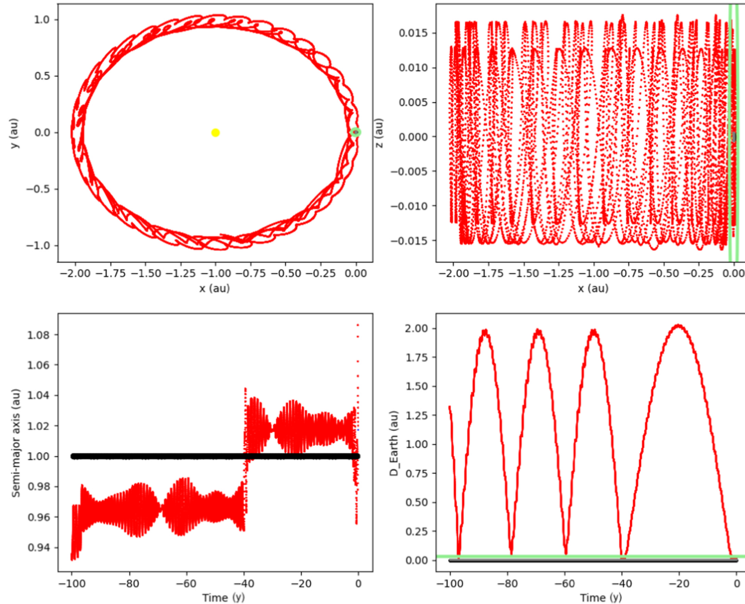
Figure 7. from Characterization of Temporarily Captured Minimoons 2020 CD3 by Keck Time-resolved Spectrophotometry null 2020 APJL 900 L45 doi:10.3847/2041-8213/abae69 https://dx.doi.org/10.3847/2041-8213/abae69 © 2020. The American Astronomical Society. All rights reserved.
