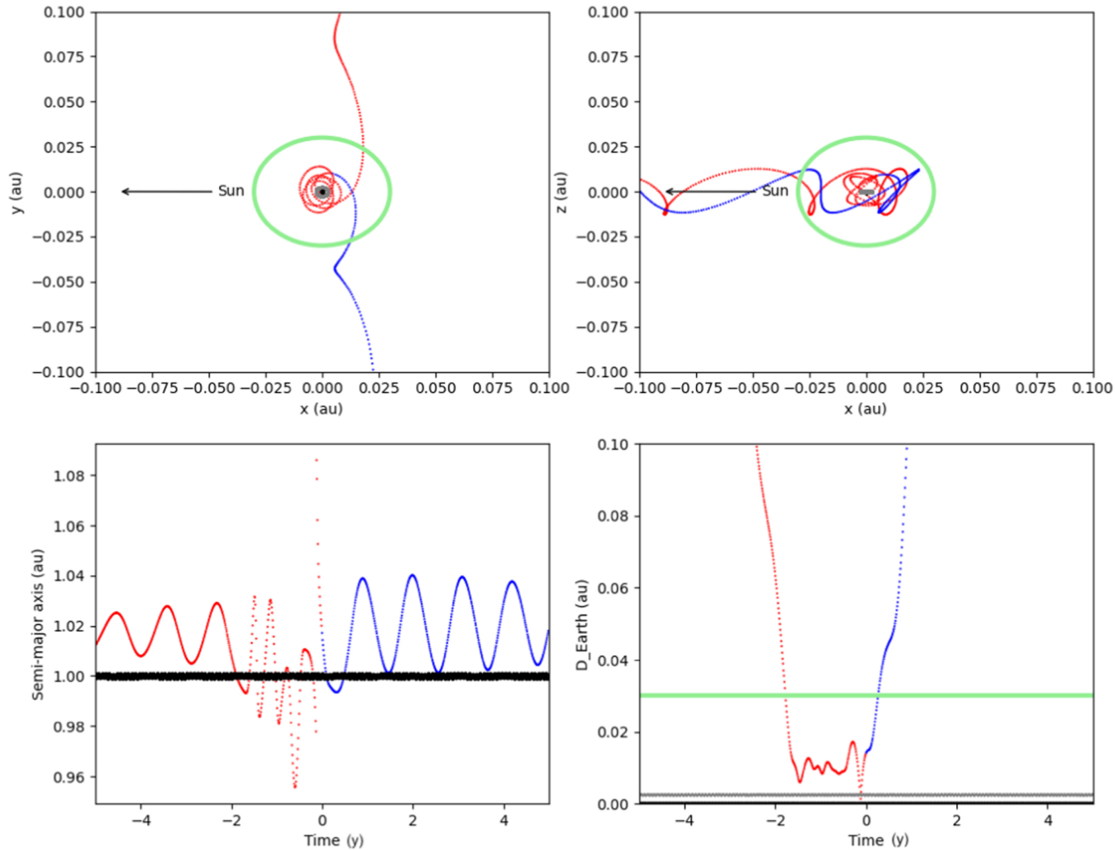
Figure 6. from Characterization of Temporarily Captured Minimoons 2020 CD3 by Keck Time-resolved Spectrophotometry null 2020 APJL 900 L45 doi:10.3847/2041-8213/abae69 https://dx.doi.org/10.3847/2041-8213/abae69
