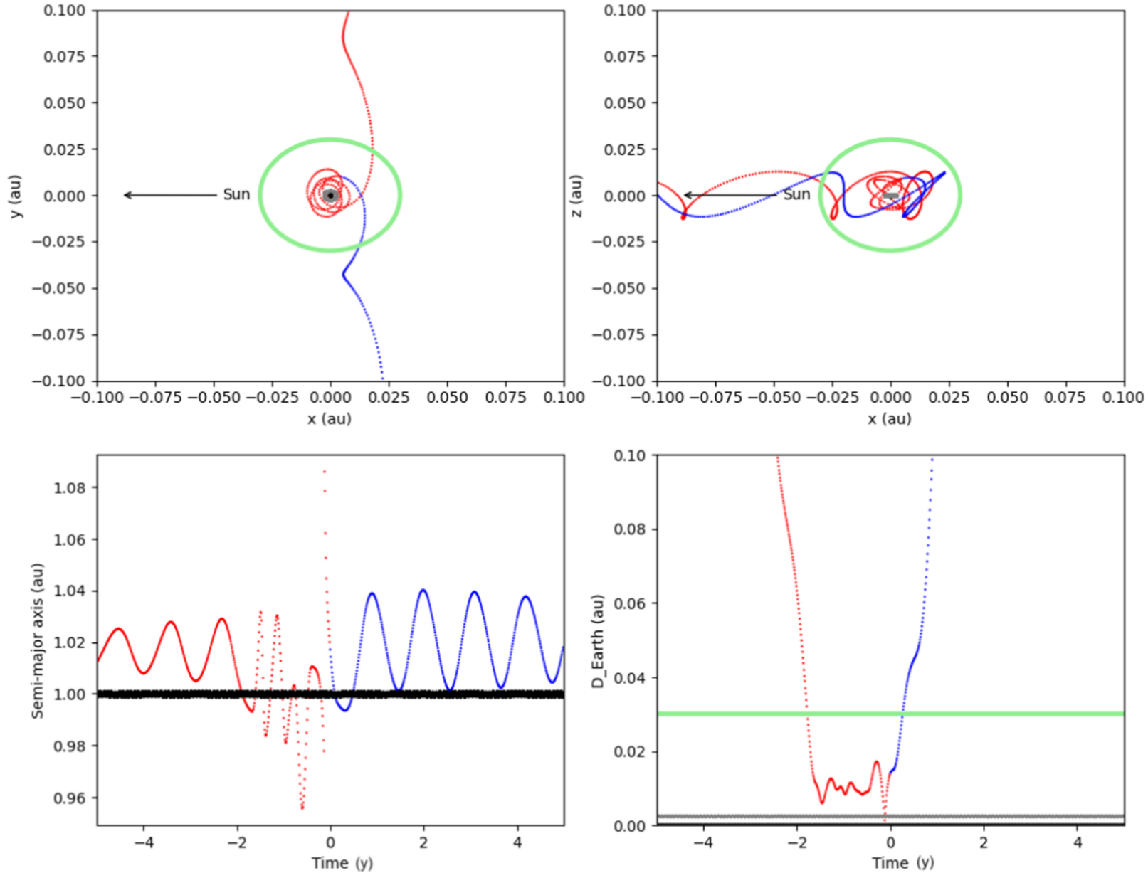
Figure 6. from Characterization of Temporarily Captured Minimoon 2020 CD3 by Keck Time-resolved Spectrophotometry null 2020 APJL 900 L45 doi:10.3847/2041-8213/abae69 http://dx.doi.org/10.3847/2041-8213/abae69
