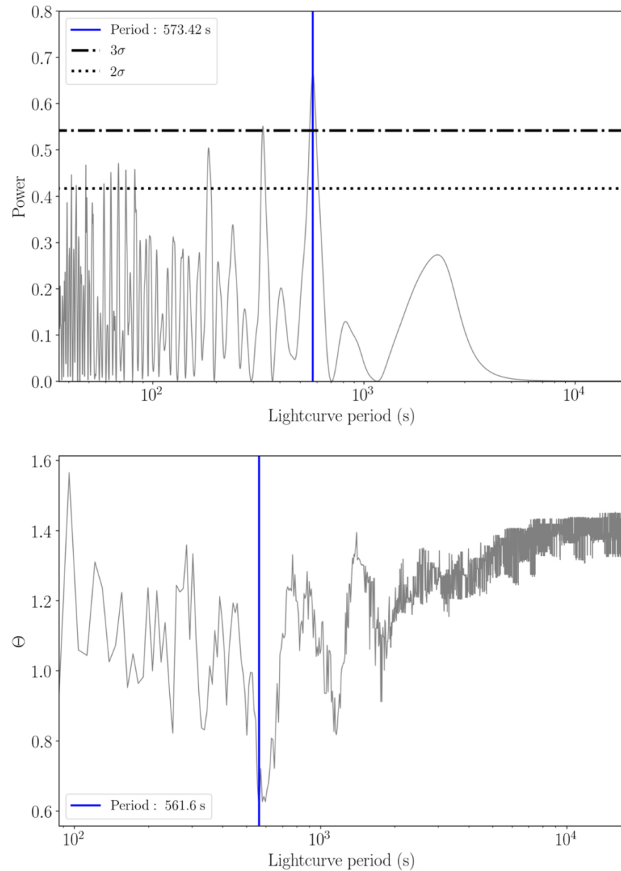
Figure 5. from Characterization of Temporarily Captured Minimoon 2020 CD3 by Keck Time-resolved Spectrophotometry null 2020 APJL 900 L45 doi:10.3847/2041-8213/abae69 https://dx.doi.org/10.3847/2041-8213/abae69
