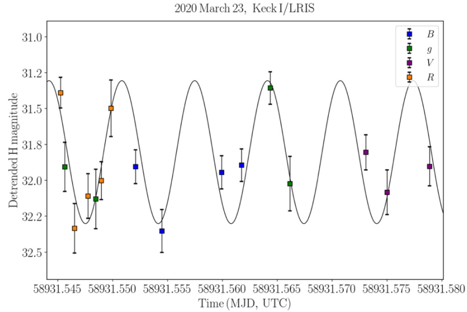
Figure 4. from Characterization of Temporarily Captured Minimoon 2020 CD3 by Keck Time-resolved Spectrophotometry null 2020 APJL 900 L45 doi:10.3847/2041-8213/abae69 http://dx.doi.org/10.3847/2041-8213/abae69 © 2020. The American Astronomical Society. All rights reserved.
