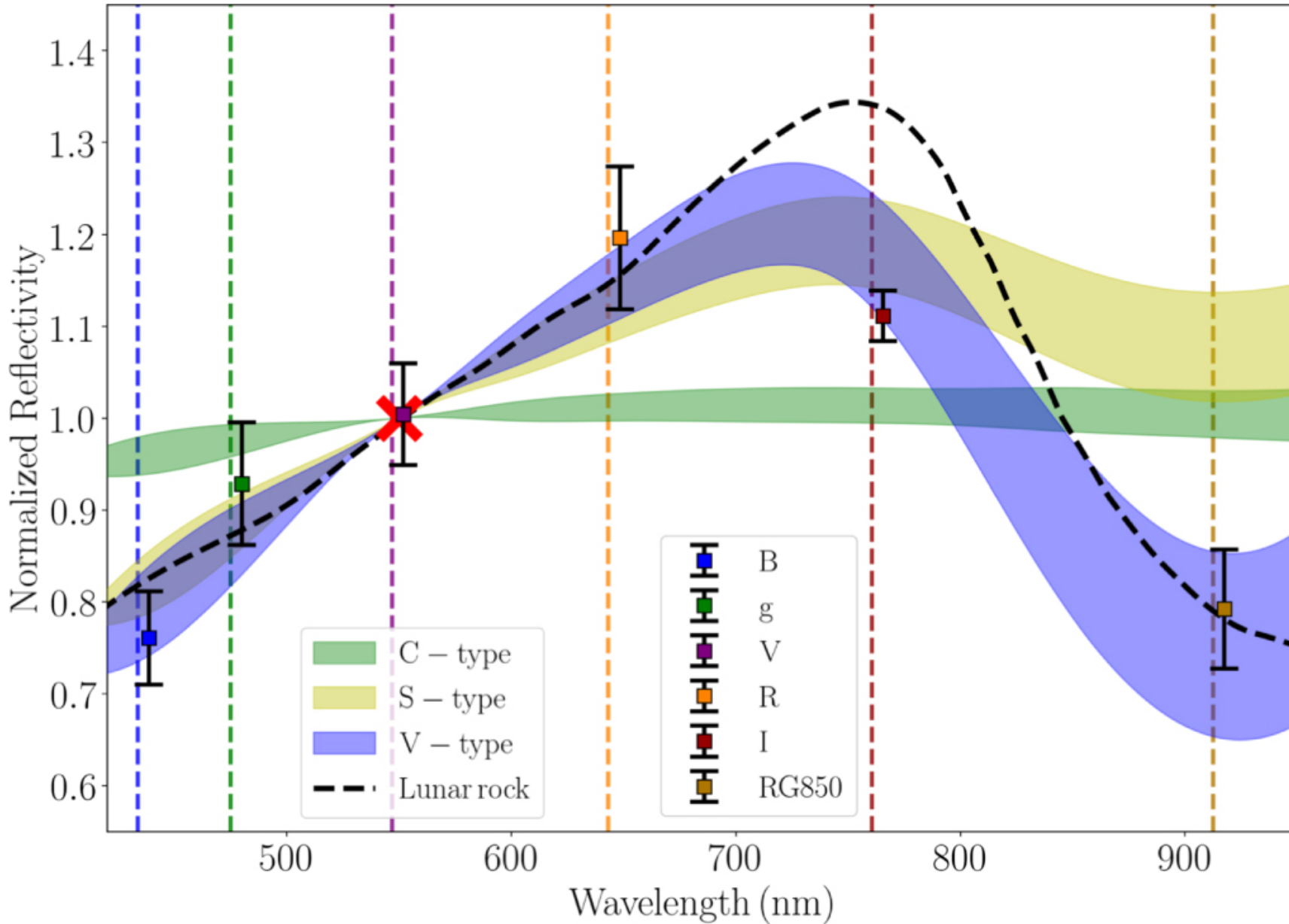
Figure 3. from Characterization of Temporarily Captured Minimoon 2020 CD3 by Keck Time-resolved Spectrophotometry null 2020 APJL 900 L45 doi:10.3847/2041-8213/abae69 http://dx.doi.org/10.3847/2041-8213/abae69 © 2020. The American Astronomical Society. All rights reserved.
