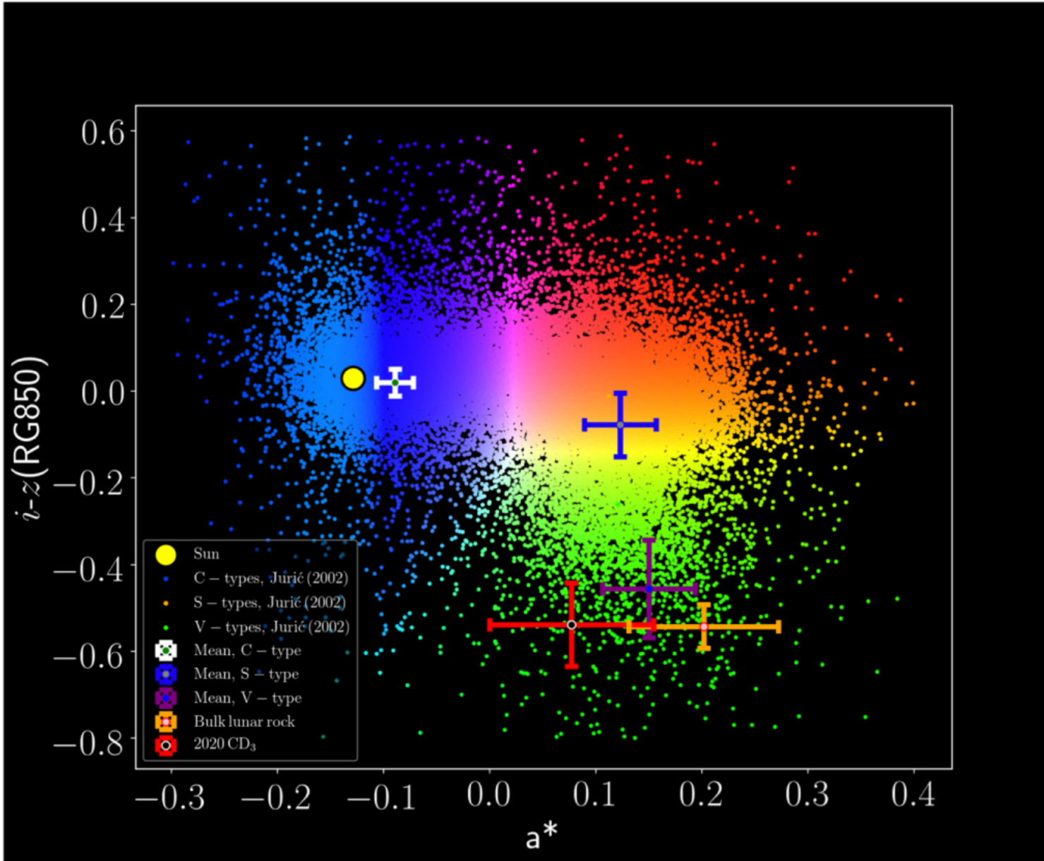
Figure 2. from Characterization of Temporarily Captured Minimoon 2020 CD3 by Keck Time-resolved Spectrophotometry null 2020 APJL 900 L45 doi:10.3847/2041-8213/abae69 http://dx.doi.org/10.3847/2041-8213/abae69 © 2020. The American Astronomical Society. All rights reserved.
