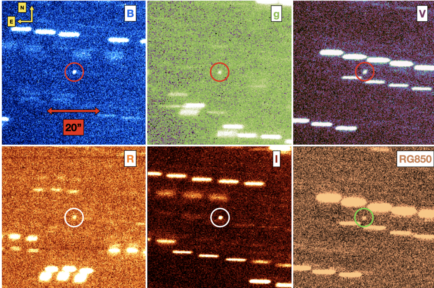
Figure 1. from Characterization of Temporarily Captured Minimoon 2020 CD3 by Keck Time-resolved Spectrophotometry null 2020 APJL 900 L45 doi:10.3847/2041-8213/abae69 https://dx.doi.org/10.3847/2041-8213/abae69 © 2020. The American Astronomical Society. All rights reserved.
