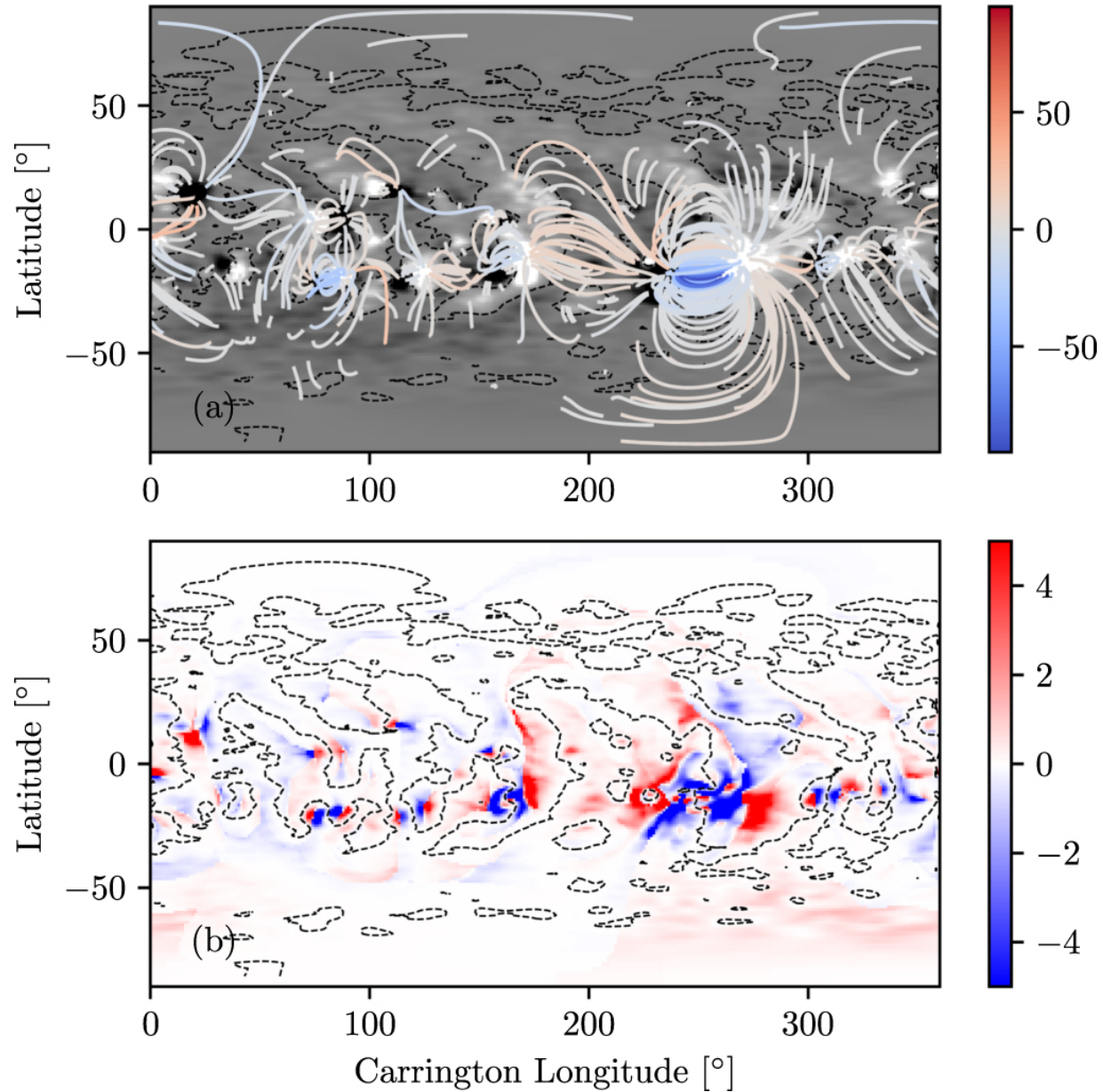
Figure 5. from The Minimal Helicity of Solar Coronal Magnetic Fields null 2020 APJL 898 L49 doi:10.3847/2041-8213/aba762 http://dx.doi.org/10.3847/2041-8213/aba762 © 2020. The American Astronomical Society. All rights reserved.
