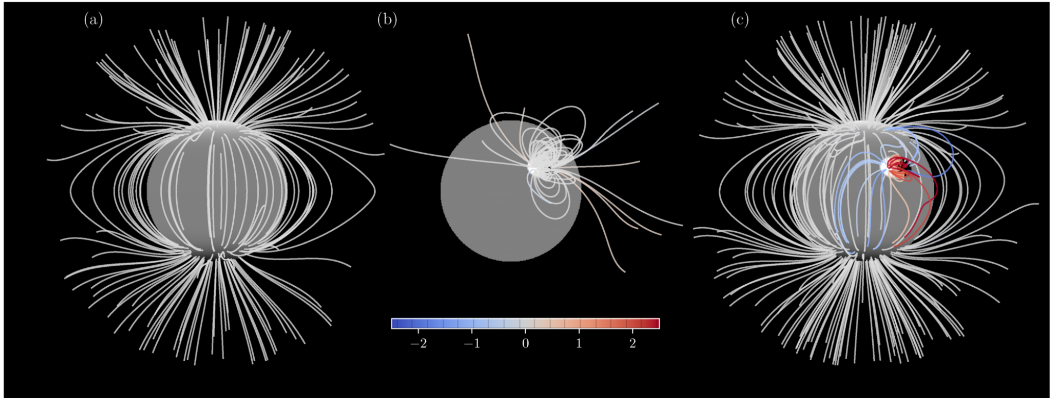
Figure 1. from The Minimal Helicity of Solar Coronal Magnetic Fields null 2020 APJL 898 L49 doi:10.3847/2041-8213/aba762 http://dx.doi.org/10.3847/2041-8213/aba762 © 2020. The American Astronomical Society. All rights reserved.
