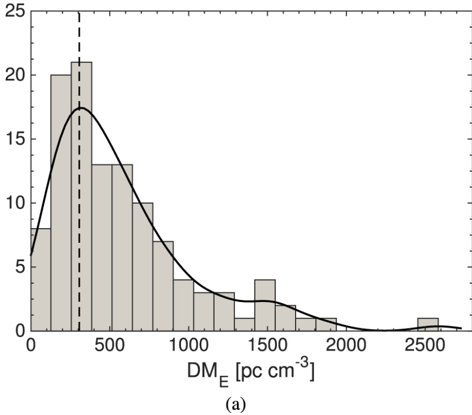
Figure 4. from Probing the Intergalactic Turbulence with Fast Radio Bursts null 2020 APJL 898 L48 doi:10.3847/2041-8213/aba760 http://dx.doi.org/10.3847/2041-8213/aba760 © 2020. The Author(s). Published by the American Astronomical Society.
