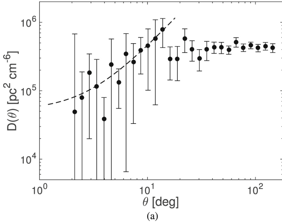
Figure 3. from Probing the Intergalactic Turbulence with Fast Radio Bursts null 2020 APJL 898 L48 doi:10.3847/2041-8213/aba760 http://dx.doi.org/10.3847/2041-8213/aba760 © 2020. The Author(s). Published by the American Astronomical Society.
