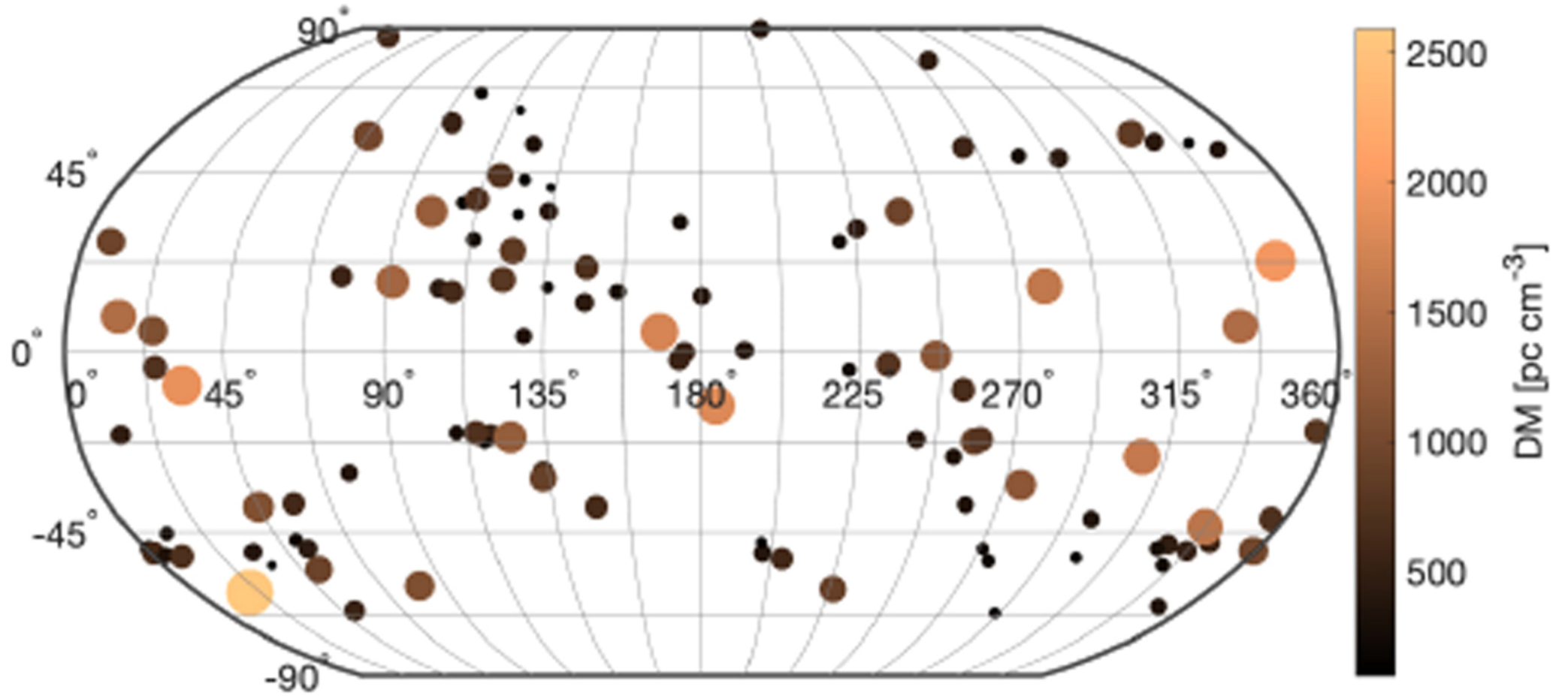
Figure 2. from Probing the Intergalactic Turbulence with Fast Radio Bursts null 2020 APJL 898 L48 doi:10.3847/2041-8213/aba760 http://dx.doi.org/10.3847/2041-8213/aba760 © 2020. The Author(s). Published by the American Astronomical Society.
