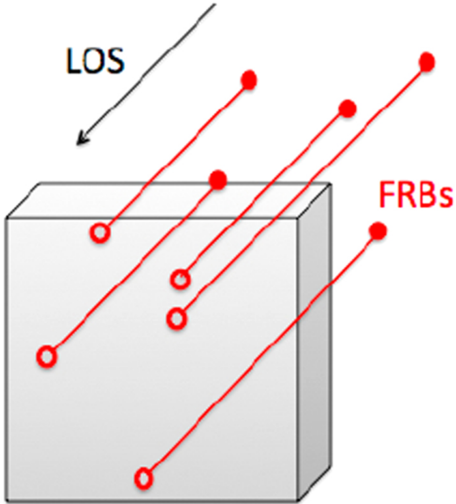
Figure 1. from Probing the Intergalactic Turbulence with Fast Radio Bursts null 2020 APJL 898 L48 doi:10.3847/2041-8213/aba760 http://dx.doi.org/10.3847/2041-8213/aba760 © 2020. The Author(s). Published by the American Astronomical Society.
